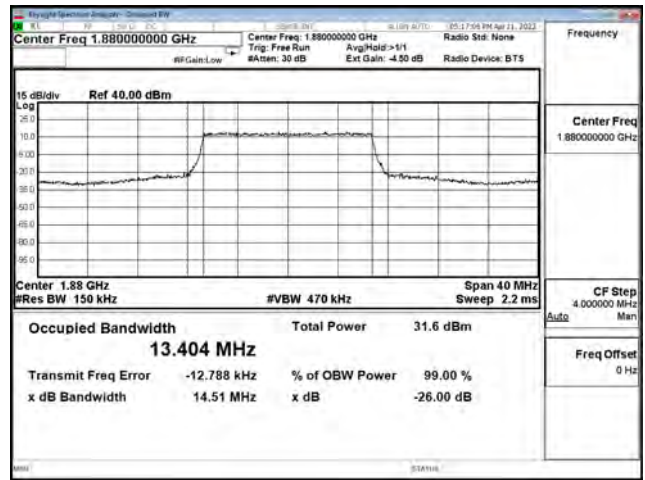
16QAM_CH18675_15M_75RB0
