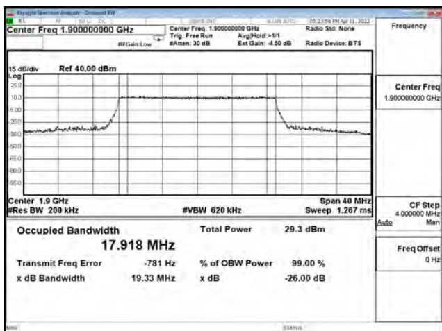
256-QAM_CH18900_20M_100RB0
