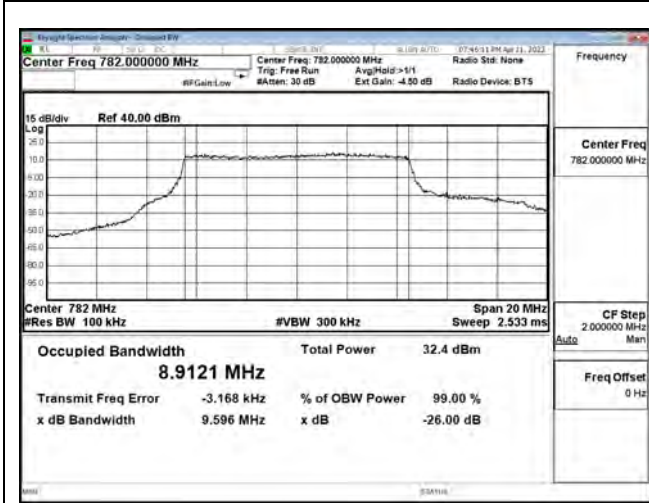
QPSK_CH23230_10M_50RB
