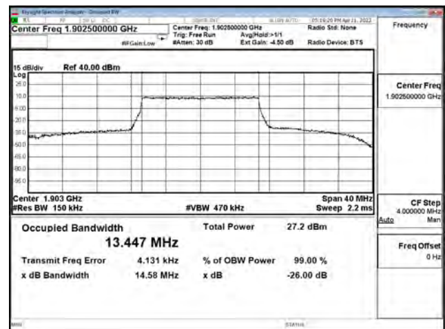
256-QAM_CH19125_15M_75RB0
