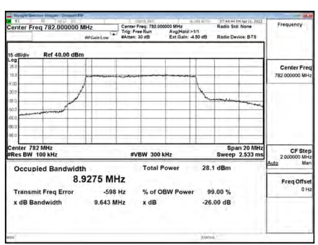
256-QAM_CH23230_10M_50RB0
