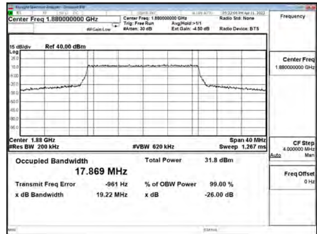
16QAM_CH18700_20M_100RB0
