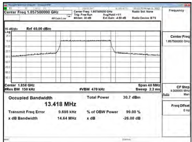
16QAM_CH19125_15M_75RB0
