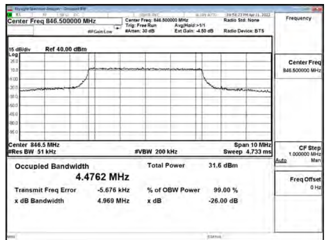
16-QAM_CH20625_5M_25RB0
