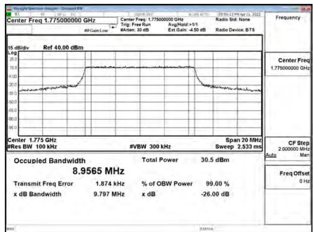
16-QAM_CH132622_10M_50RB0
