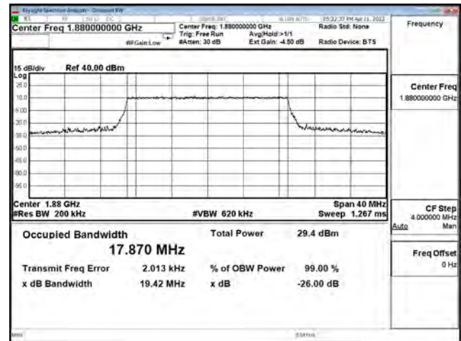
256-QAM_CH18700_20M_100RB0
