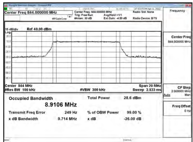
256-QAM_CH20600_10M_50RB0
