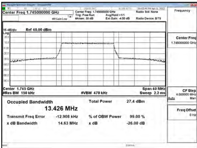
256-QAM_CH132322_15M_75RB0
