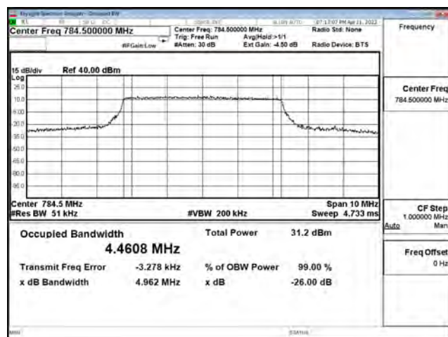
16-QAM_CH23255_5M_25RB0
