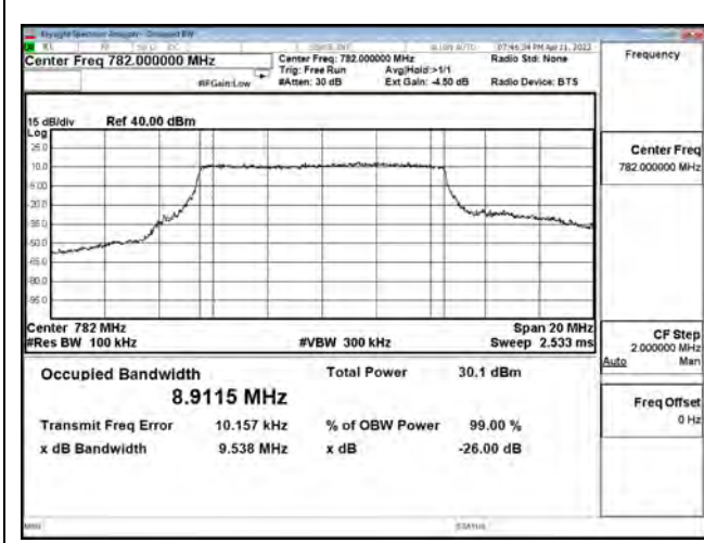
64-QAM_CH23230_10M_50RB0
