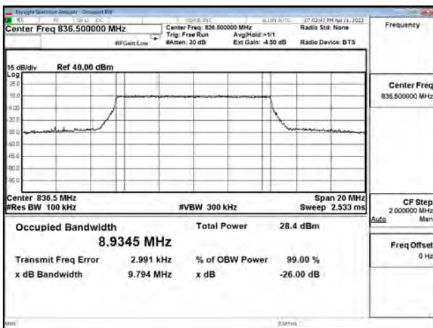
256-QAM_CH20525_10M_50RB0
