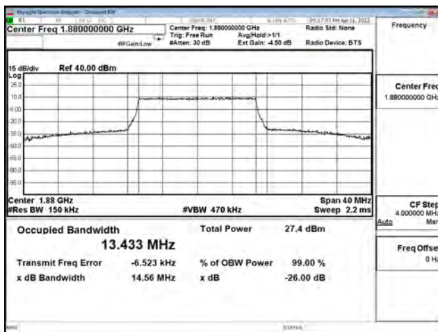
256-QAM_CH18900_15M_75RB0
