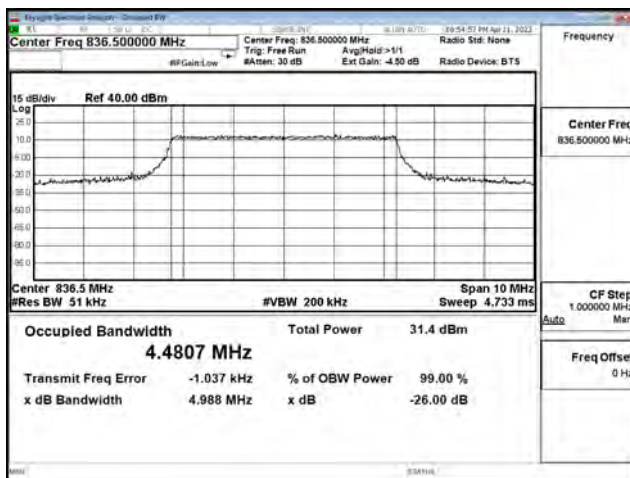
16-QAM_CH20525_5M_25RB0
