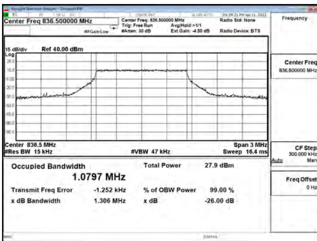
256-QAM_CH20525_1.4M_6RB0
