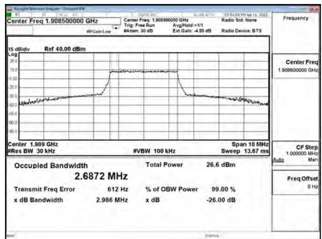
256-QAM_CH19185_3M_15RB0
