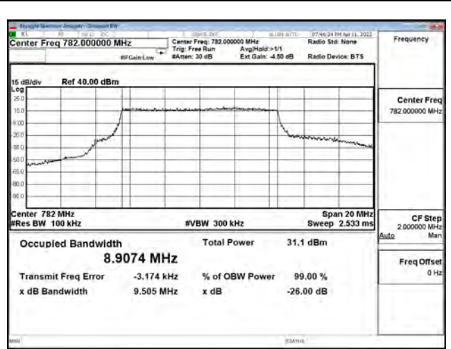
16-QAM_CH23230_10M_50RB0
