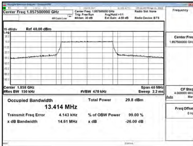
64-QAM_CH19125_15M_75RB0
