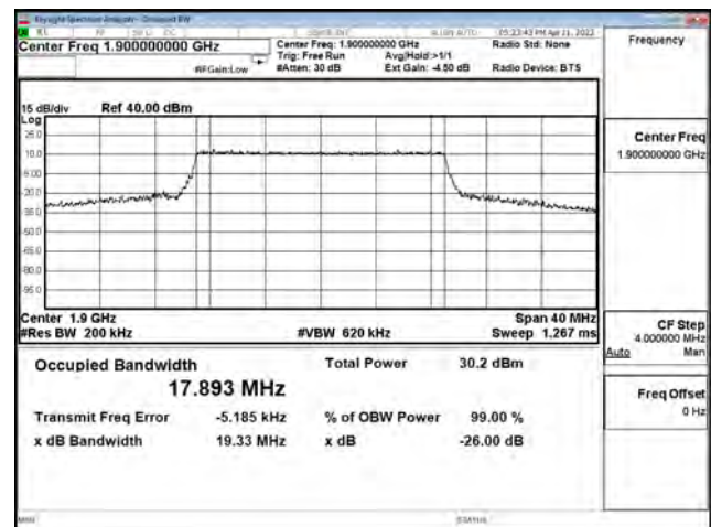
16QAM_CH19100_20M_100RB0
