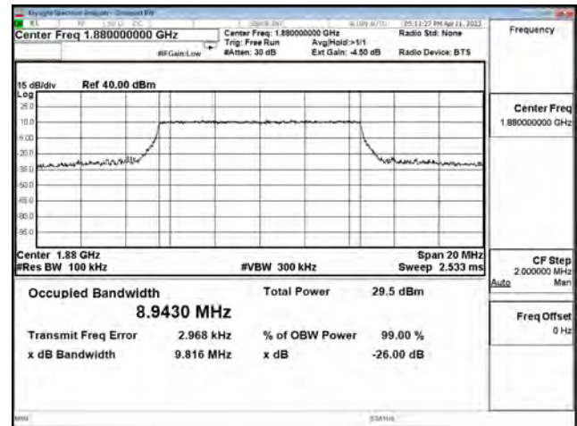
256-QAM_CH18650_10M_50RB0
