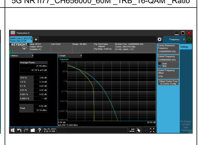
5G NR n77_CH656000_60M_1RB_16-QAM_Ratio
