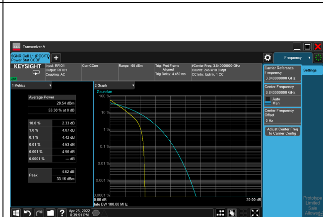
5G NR n77_CH656000_80M_1RB_pi/2 BPSK_Ratio
