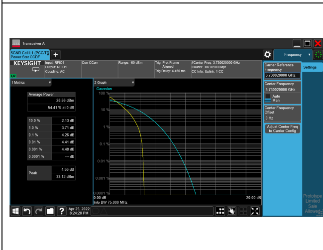
5G NR n77_CH648668_60M_1RB_16-QAM_Ratio
