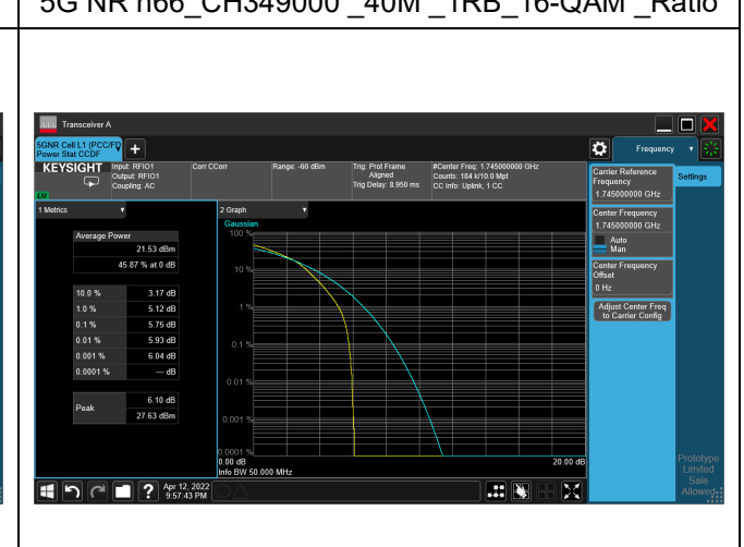
5G NR n66_CH349000_40M_1RB_16-QAM_Ratio
