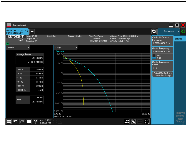
5G NR n66_CH346000_40M_1RB_16-QAM_Ratio
