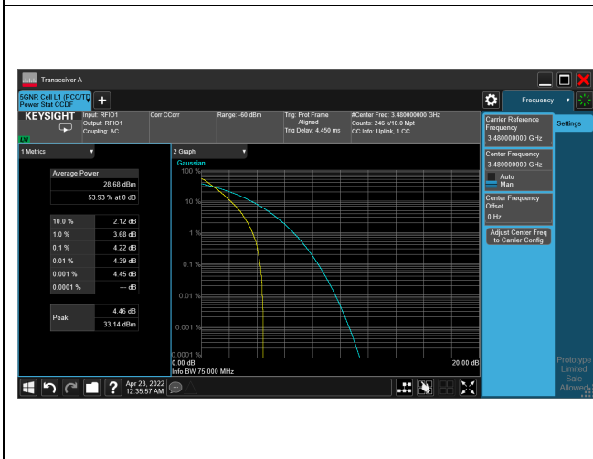
5G NR n77_CH632000_60M_1RB_16-QAM_Ratio
