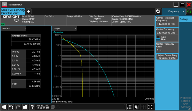
5G NR n77_CH631666_50M_1RB_16-QAM_Ratio
