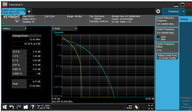
5G NR n5_CH166300_15M_1RB_16-QAM_Ratio
