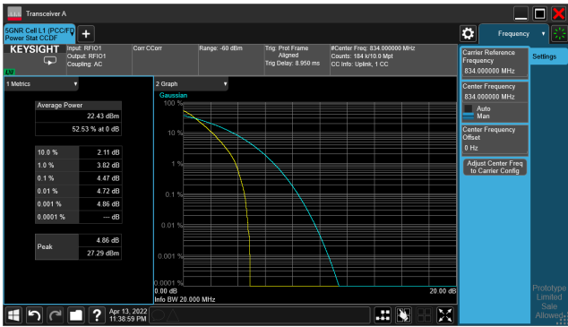
5G NR n5_CH166800_20M_1RB_16-QAM_Ratio
