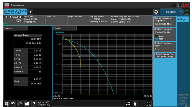
5G NR n5_CH167300_5M_1RB_16-QAM_Ratio
