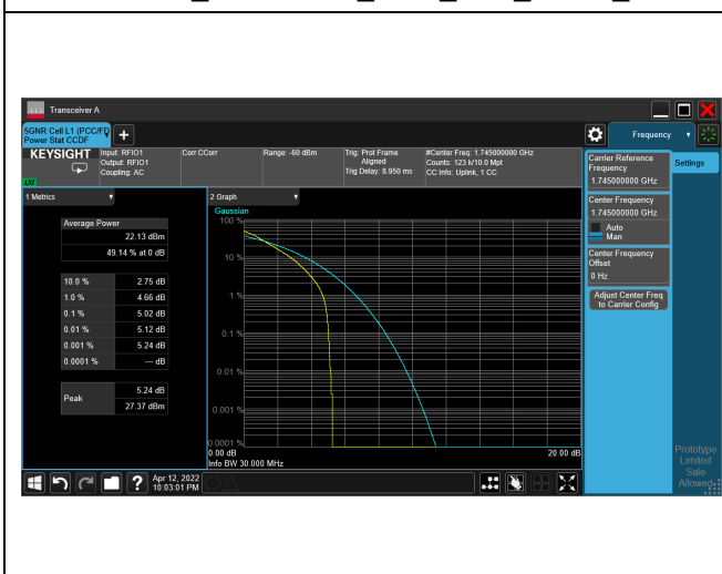
5G NR n66_CH349000_30M_1RB_QPSK_Ratio
