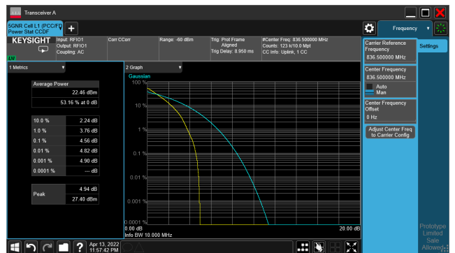
5G NR n5_CH167300_10M_1RB_16-QAM_Ratio
