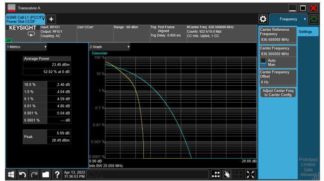
5G NR n5_CH167300_20M_1RB_16-QAM_Ratio
