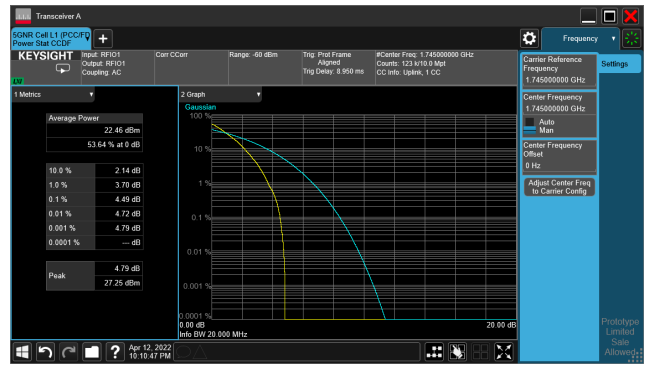
5G NR n66_CH349000_15M_1RB_16-QAM_Ratio
