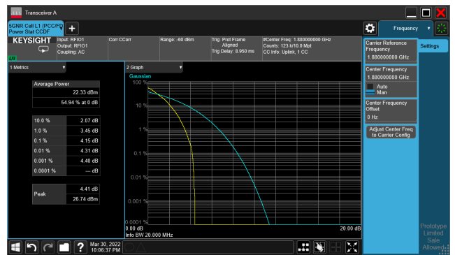
5G NR n2_CH376000_15M_1RB_16-QAM_Ratio
