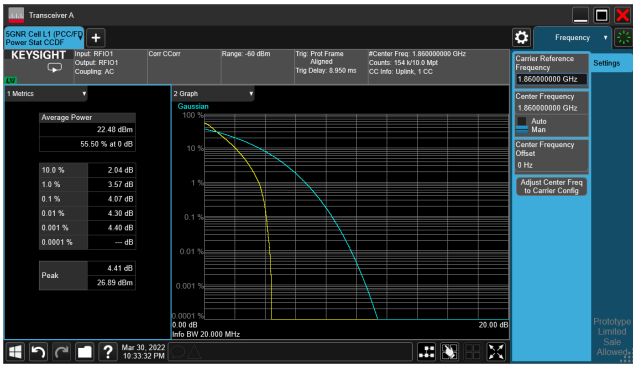
5G NR n2_CH372000_20M_1RB_16-QAM_Ratio
