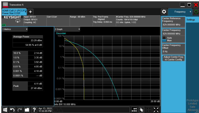
5G NR n5_CH165800_10M_1RB_16-QAM_Ratio
