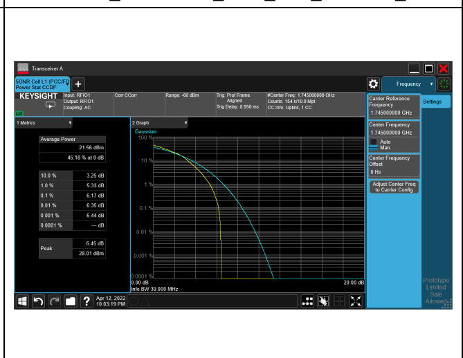
5G NR n66_CH349000_30M_1RB_16-QAM_Ratio
