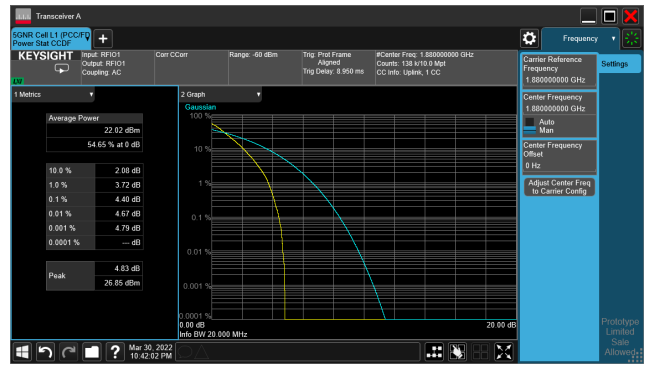
5G NR n2_CH376000_20M_1RB_16-QAM_Ratio
