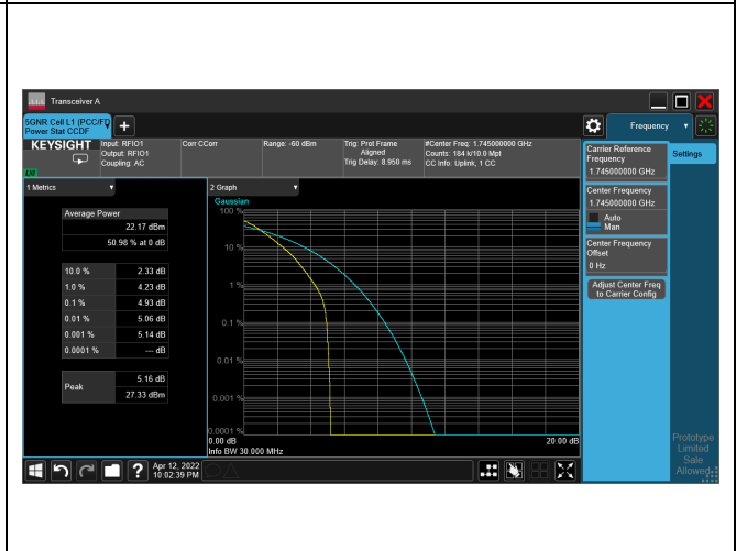
5G NR n66_CH349000_30M_1RB_16-QAM_Ratio
