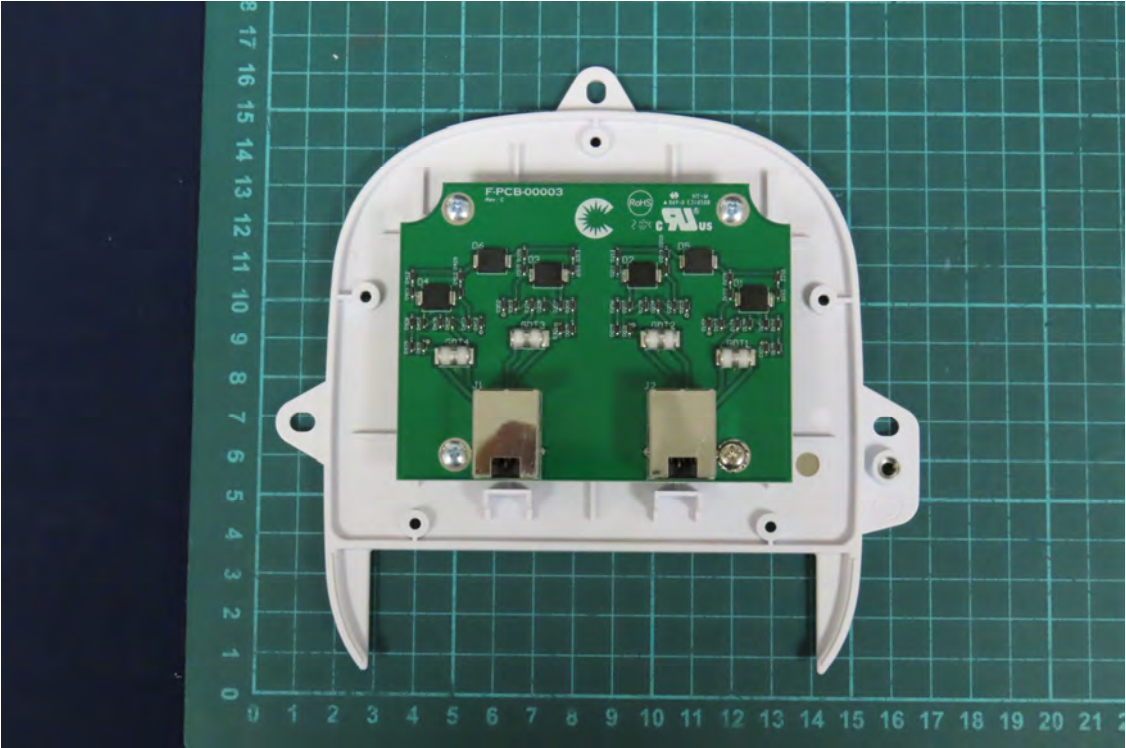
(73) EUT Photo
