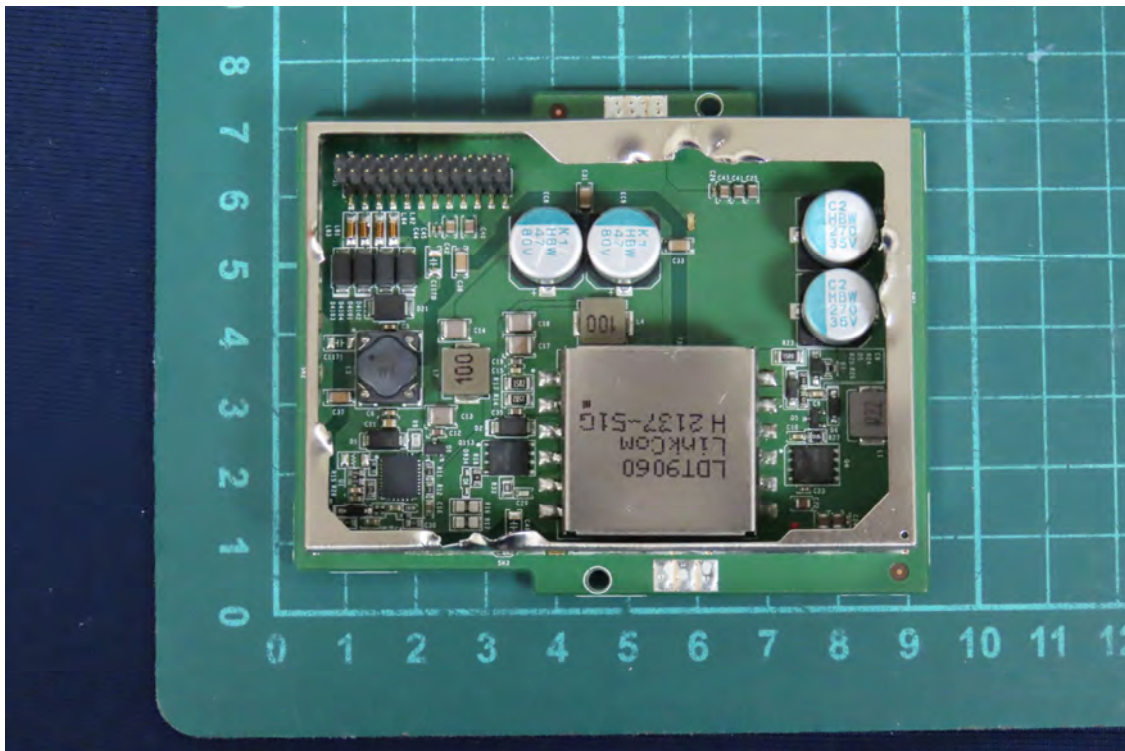
(45) EUT Photo
