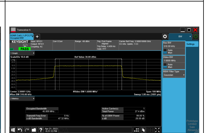
16QAM_CH633334_50M
