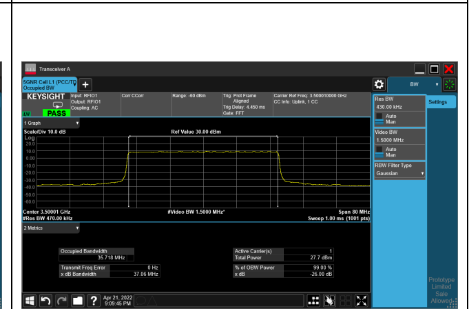
16QAM_CH633334_40M
