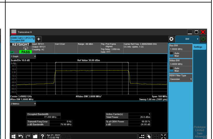
64QAM_CH632668_80M
