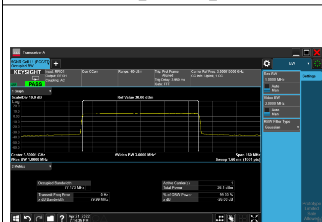
64QAM_CH633334_80M
