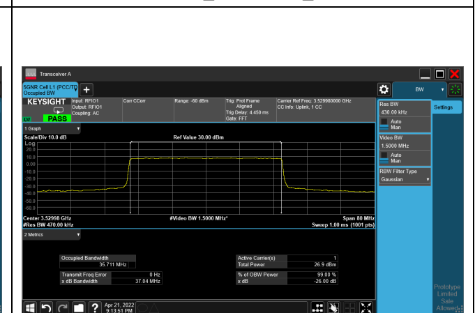
64QAM_CH635332_40M
