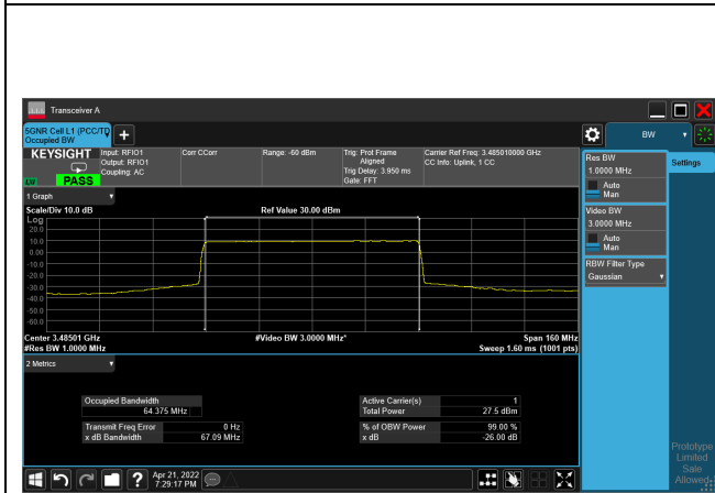
16QAM_CH632334_70M
