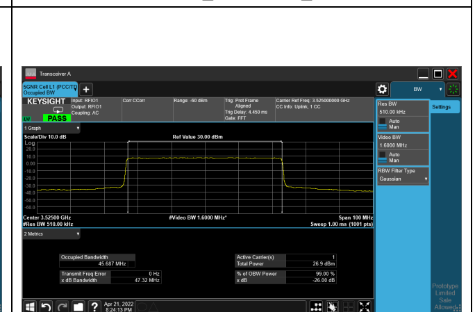
64QAM_CH635000_50M
