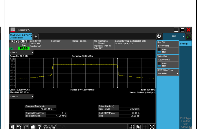
QPSK_CH635000_50M
