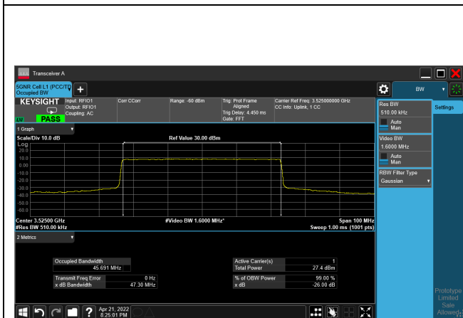
16QAM_CH635000_50M
