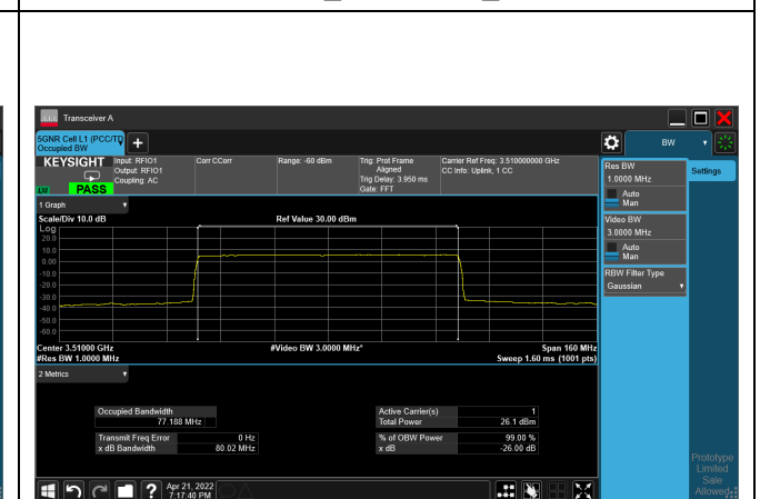
64QAM_CH634000_80M
