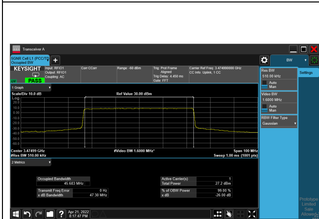
16QAM_CH631666_50M
