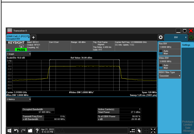
16QAM_CH634666_60M
