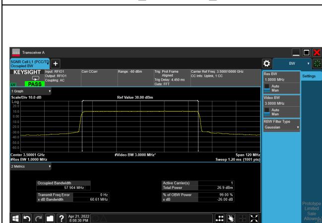
64QAM_CH633334_60M
