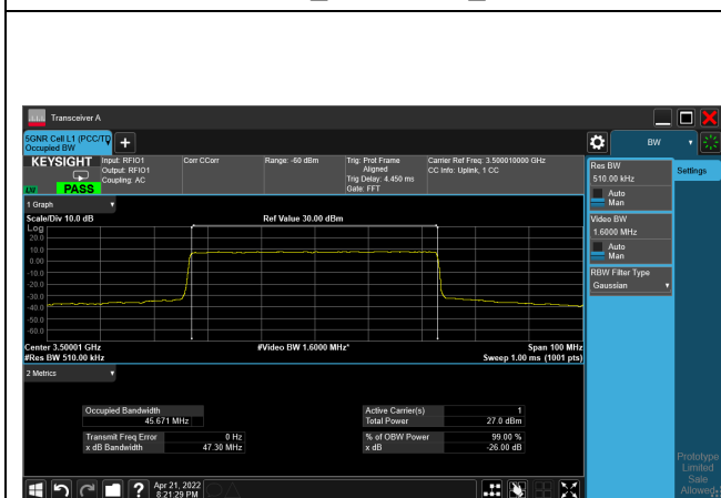
64QAM_CH633334_50M
