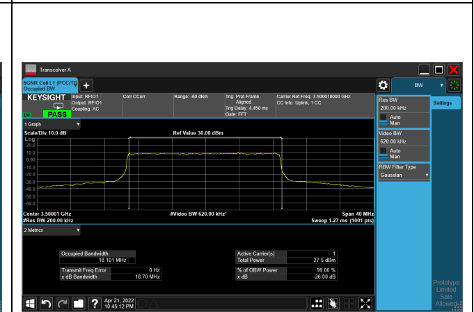
16QAM_CH633334_20M
