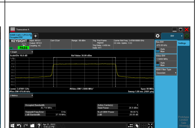
64QAM_CH631334_40M
