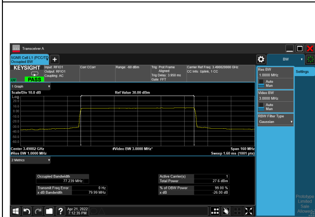
16QAM_CH632668_80M
