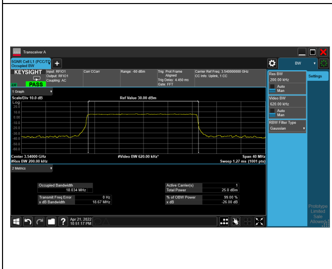
256QAM_CH636000_20M
