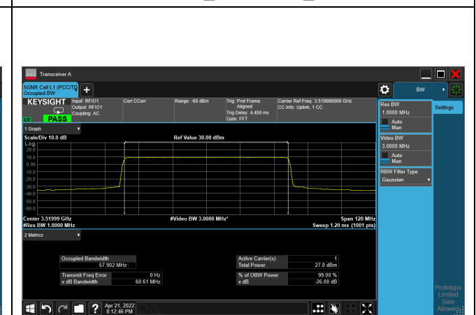
64QAM_CH634666_60M
