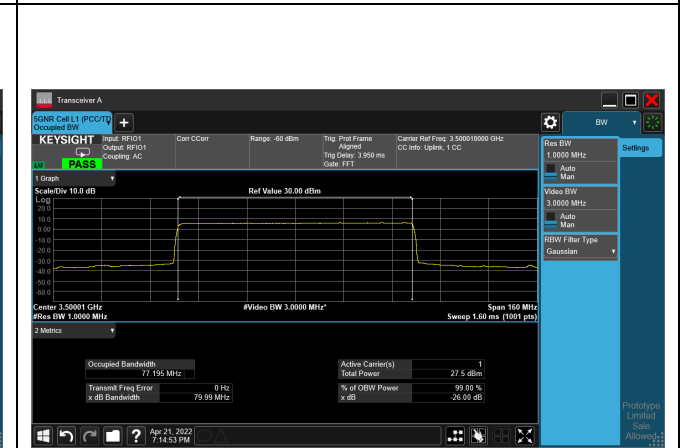
16QAM_CH633334_80M
