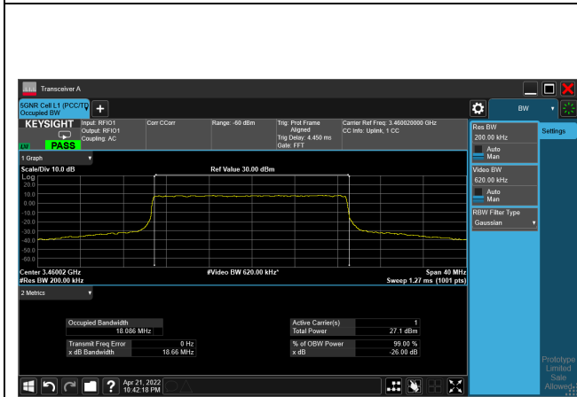
16QAM_CH630668_20M
