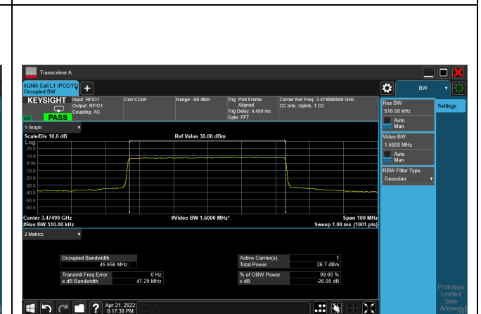
64QAM_CH631666_50M
