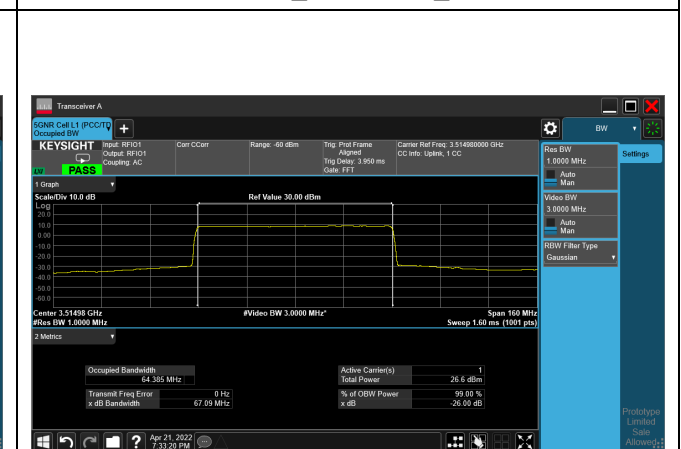
64QAM_CH634332_70M
