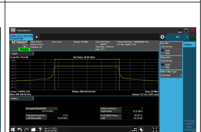
64QAM_CH630668_20M
