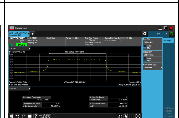
64QAM_CH636000_20M
