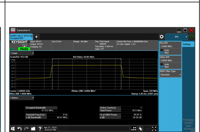
64QAM_CH632000_60M
