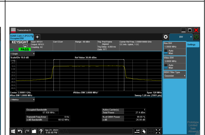
16QAM_CH633334_60M
