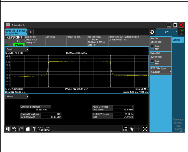
256QAM_CH349000_20M
