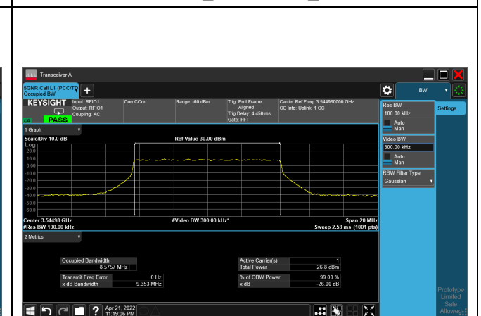
64QAM_CH636332_10M
