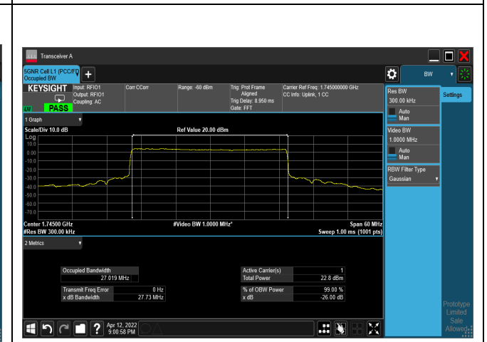
pi/2-BPSK_CH349000_30M
