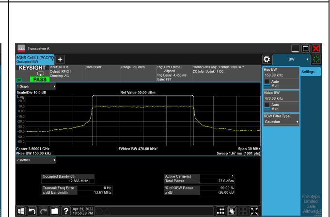
16QAM_CH633334_15M
