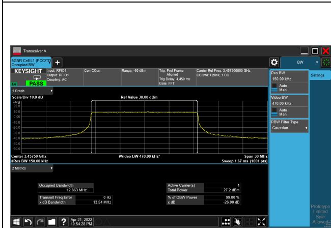
16QAM_CH630500_15M
