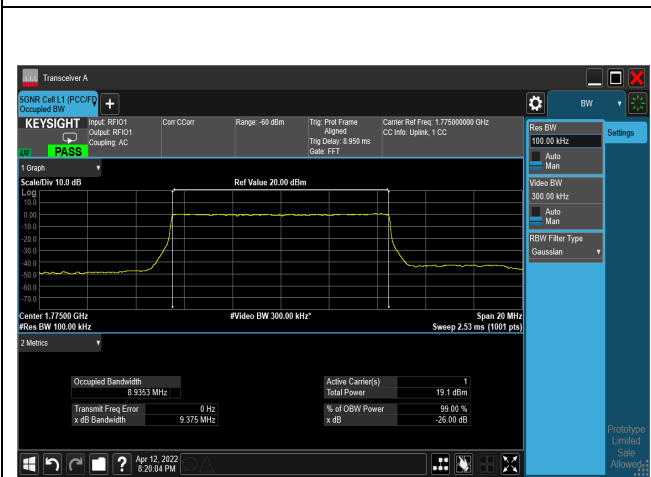
256QAM_CH355000_10M
