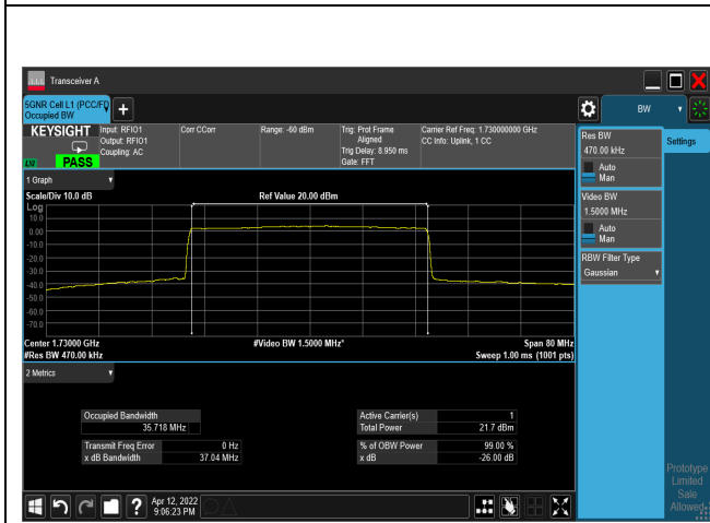
16QAM_CH346000_40M
