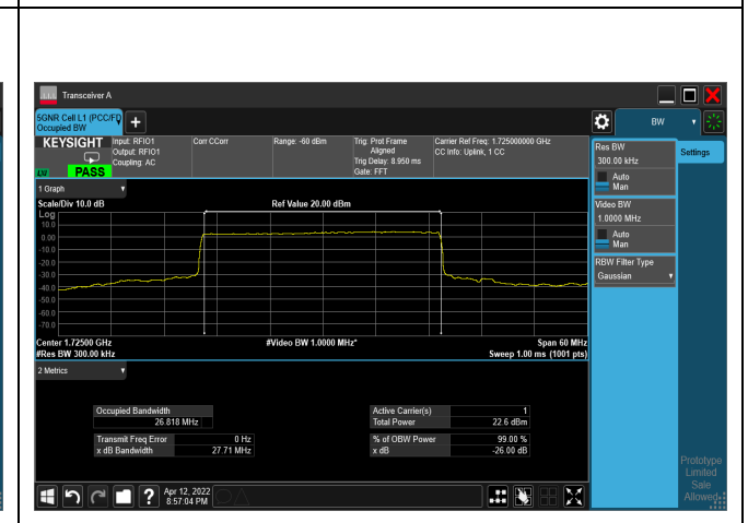
QPSK_CH345000_30M
