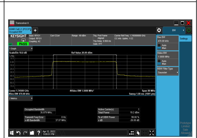
256QAM_CH349000_40M
