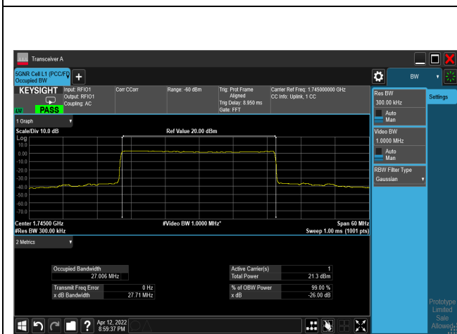
64QAM_CH349000_30M
