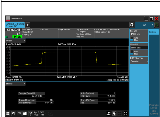
256QAM_CH346000_40M
