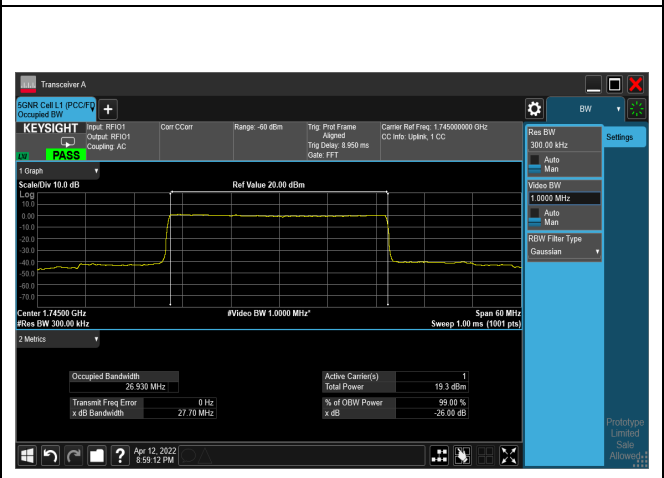
256QAM_CH349000_30M
