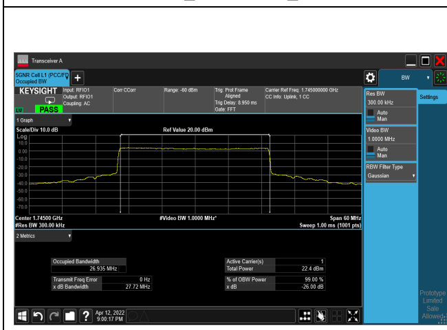
QPSK_CH349000_30M
