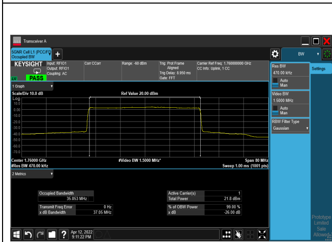
16QAM_CH352000_40M
