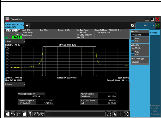
256QAM_CH343000_10M
