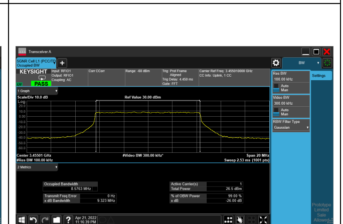
64QAM_CH630334_10M
