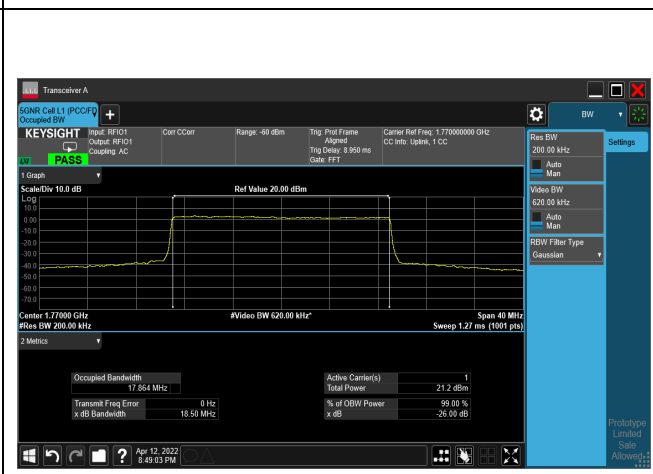
64QAM_CH354000_20M
