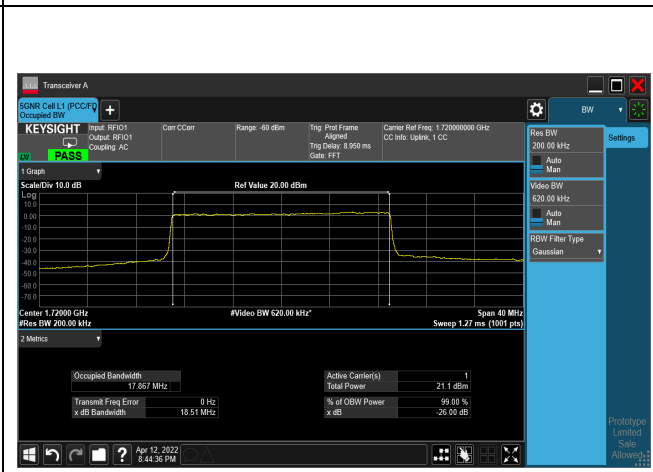
64QAM_CH344000_20M
