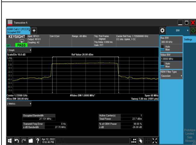
pi/2-BPSK_CH345000_30M
