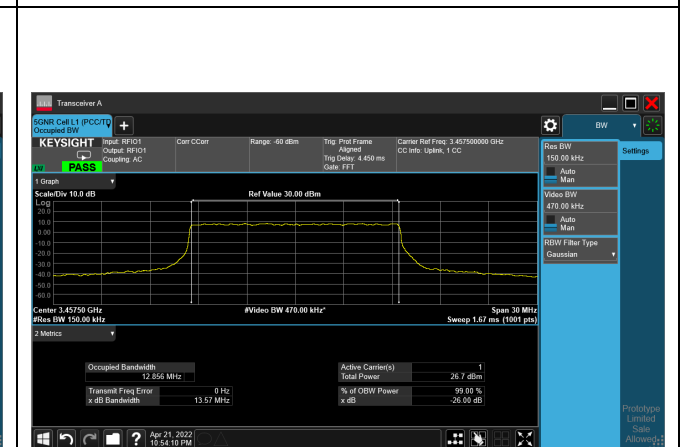
64QAM_CH630500_15M
