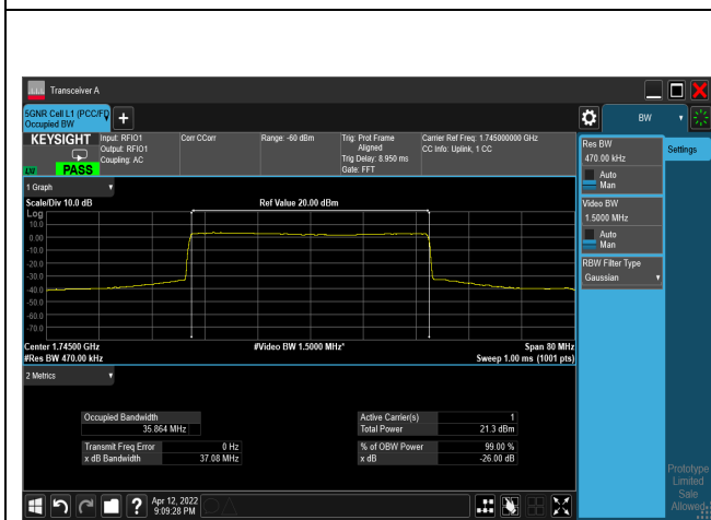
64QAM_CH349000_40M
