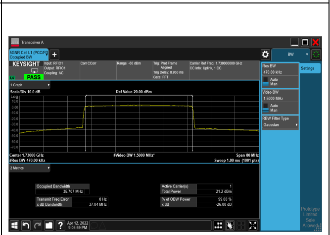
64QAM_CH346000_40M
