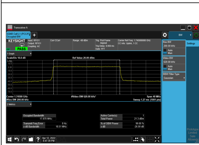
64QAM_CH349000_20M
