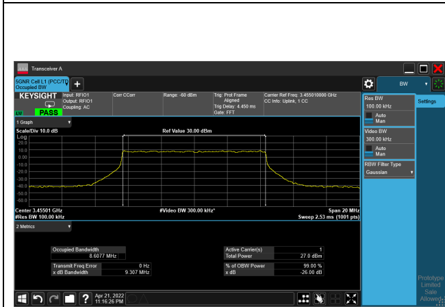
16QAM_CH630334_10M
