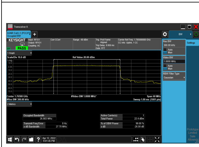
pi/2-BPSK_CH353000_30M
