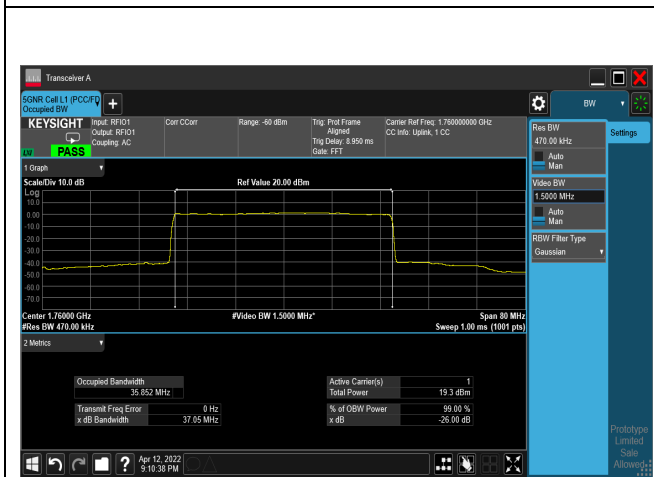
256QAM_CH352000_40M
