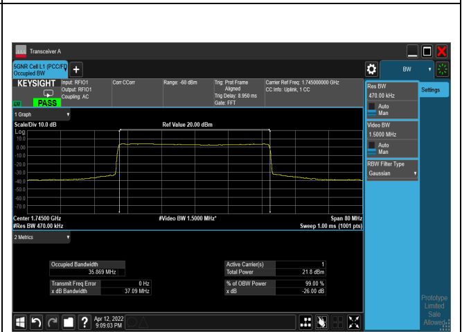
16QAM_CH349000_40M
