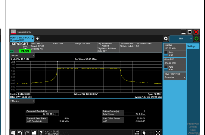
64QAM_CH636166_15M
