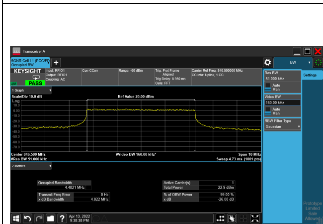
16QAM_CH169300_5M
