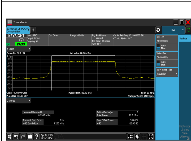
pi/2-BPSK_CH343000_10M
