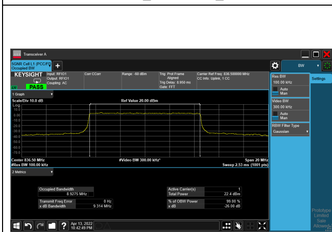
64QAM_CH167300_10M
