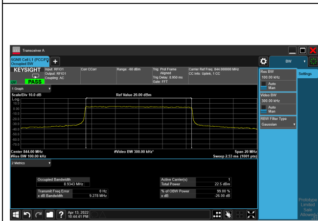
16QAM_CH168800_10M
