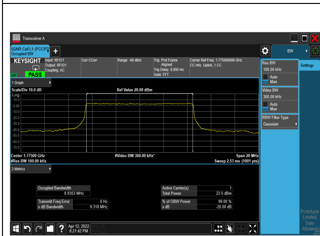
pi/2-BPSK_CH355000_10M
