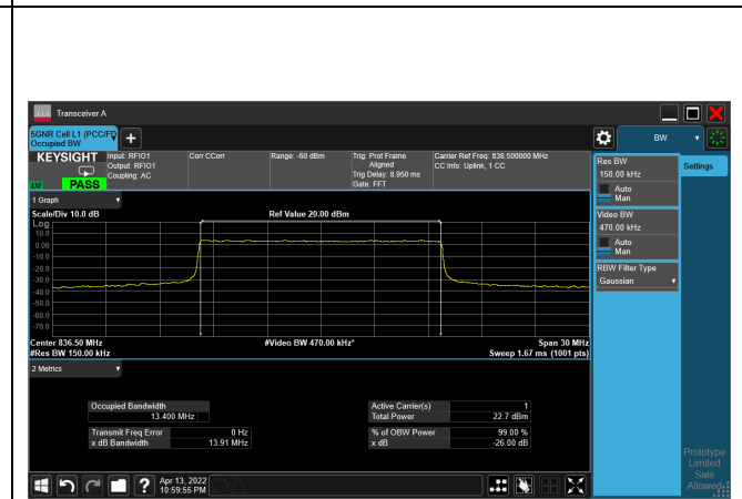
16QAM_CH167300_15M
