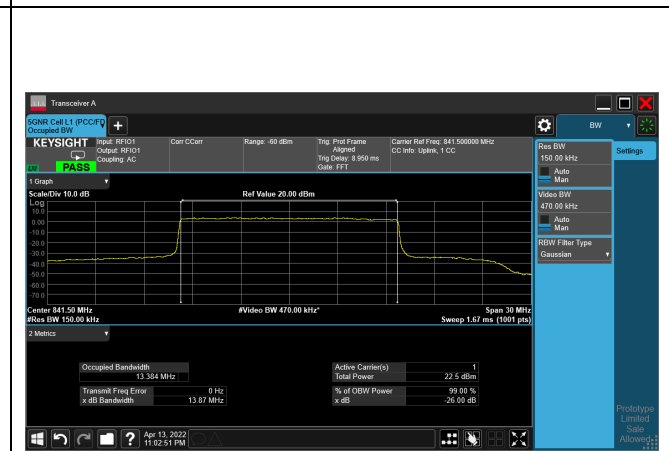
64QAM_CH168300_15M
