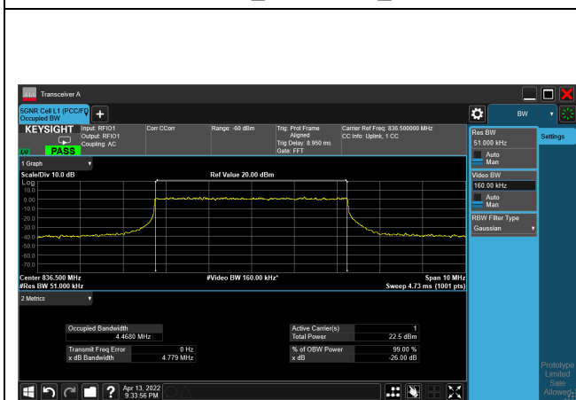
64QAM_CH167300_5M
