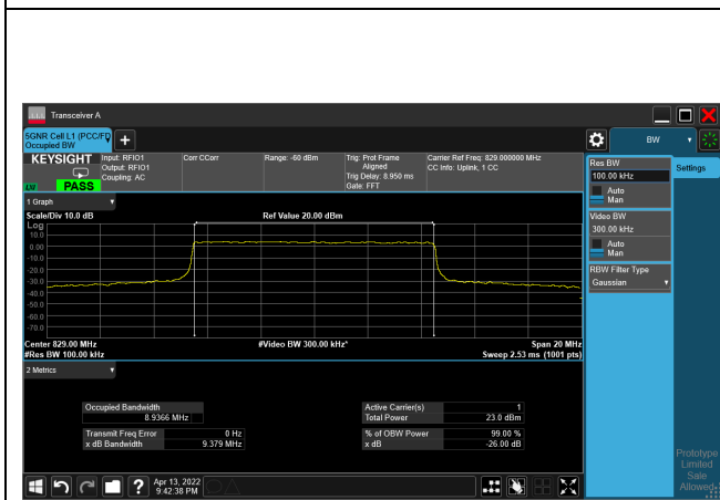
16QAM_CH165800_10M
