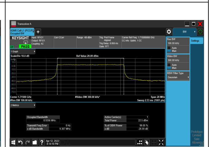
QPSK_CH343000_10M
