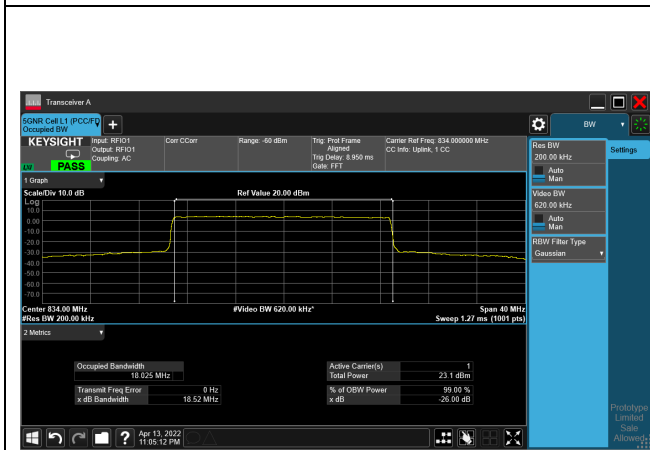
16QAM_CH166800_20M
