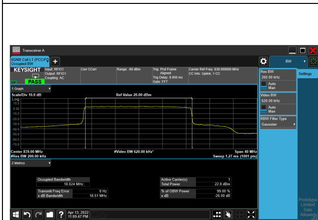
16QAM_CH167800_20M
