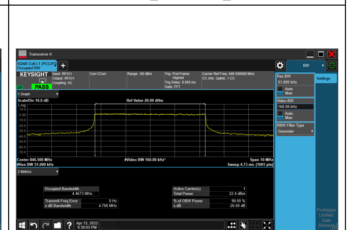
64QAM_CH169300_5M
