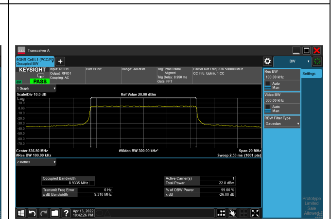
16QAM_CH167300_10M
