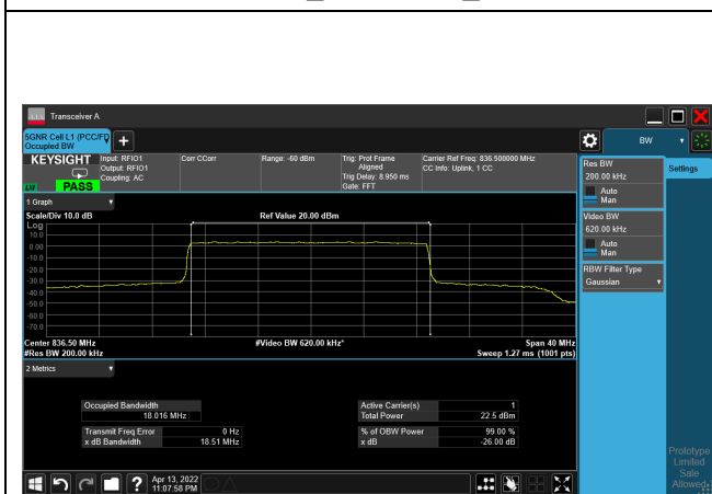
64QAM_CH167300_20M
