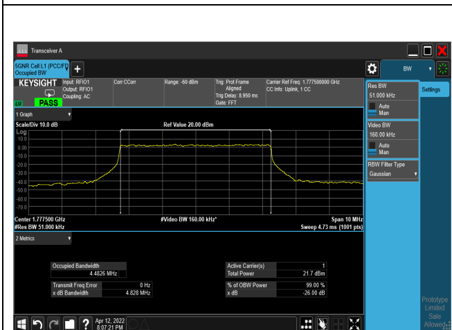
16QAM_CH355500_5M
