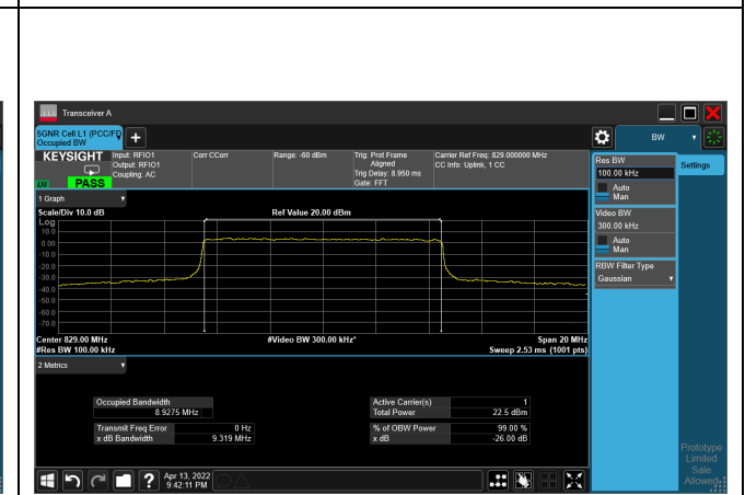
64QAM_CH165800_10M
