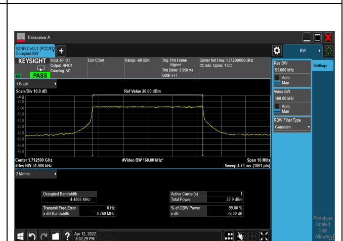
64QAM_CH342500_5M
