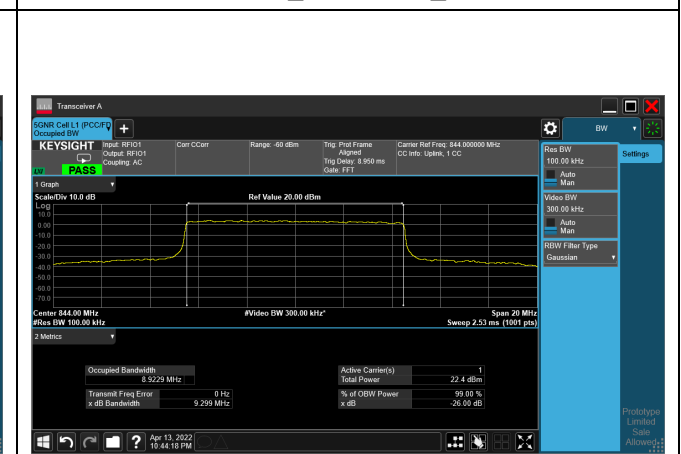
64QAM_CH168800_10M
