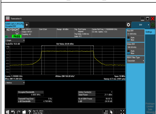
64QAM_CH349000_5M
