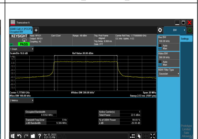
QPSK_CH355000_10M
