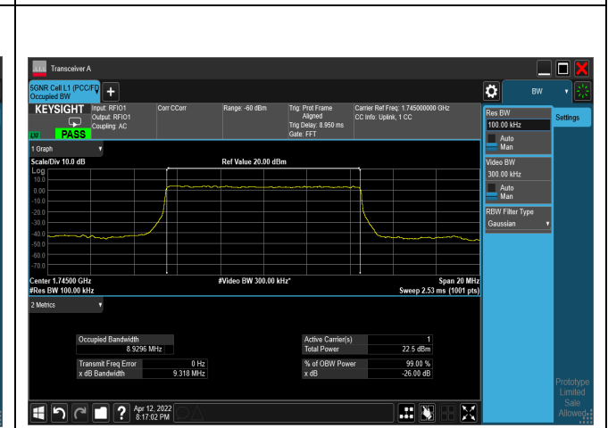
pi/2-BPSK_CH349000_10M
