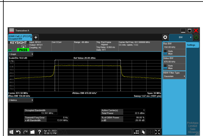
64QAM_CH166300_15M
