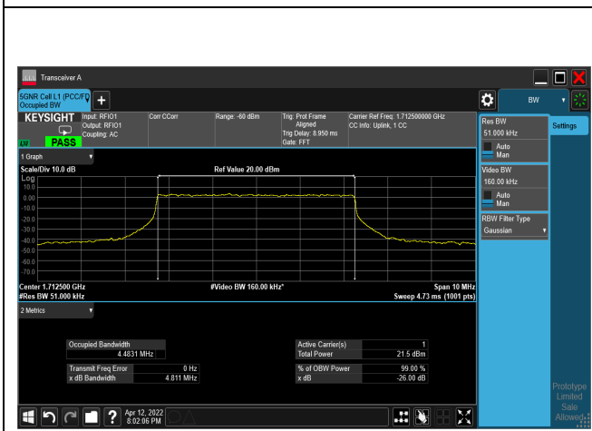
16QAM_CH342500_5M
