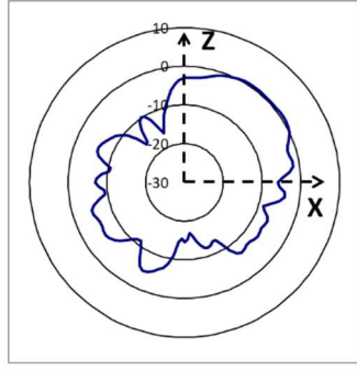
5600 MHz Radiation Pattern — S10H
