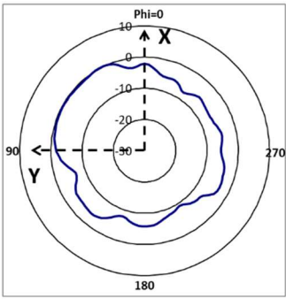
5600 MHz Radiation Pattern — S10V
