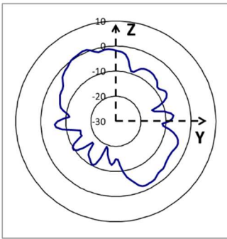
6000 MHz Radiation Pattern
