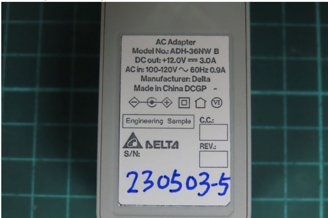
(62) EUT Photo (ADH-36NW B)
