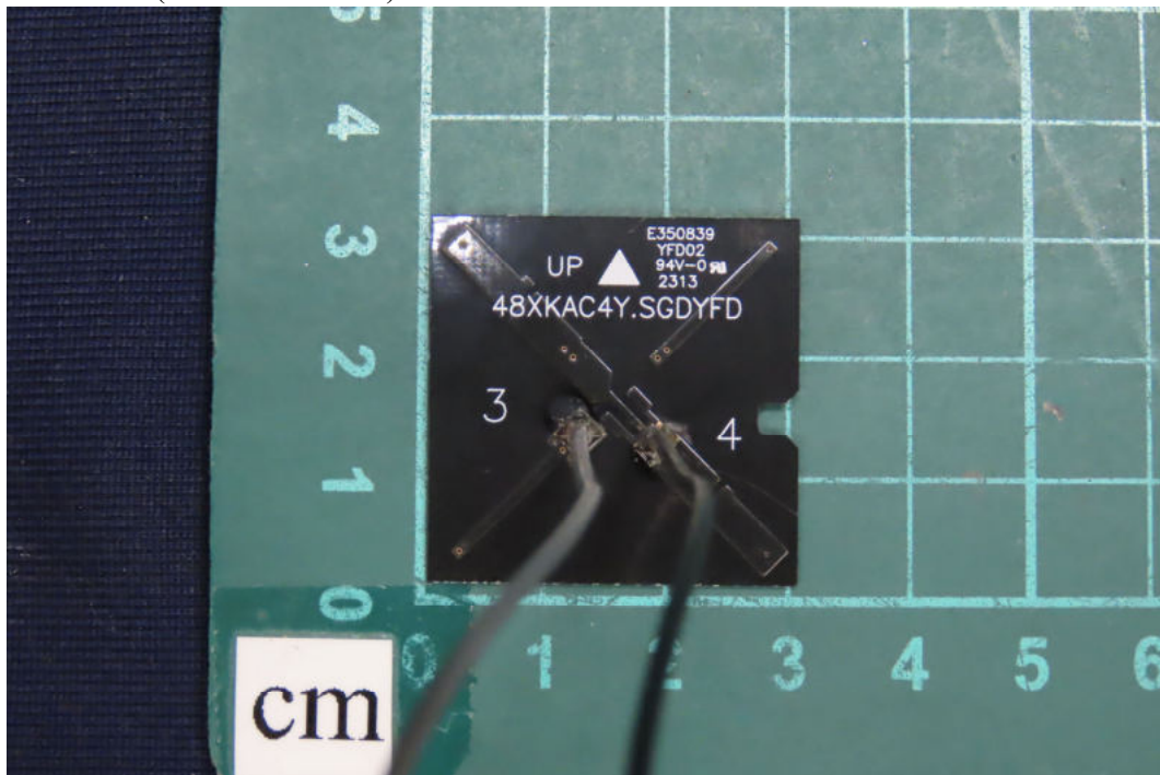
(41) EUT Photo (2.4G-5G antenna)
