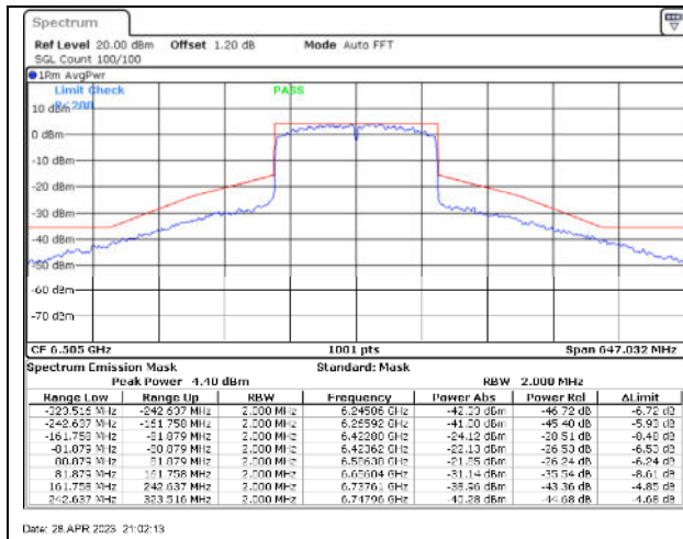
802.11ax160 / 6505MHz / Chain A - CDD
