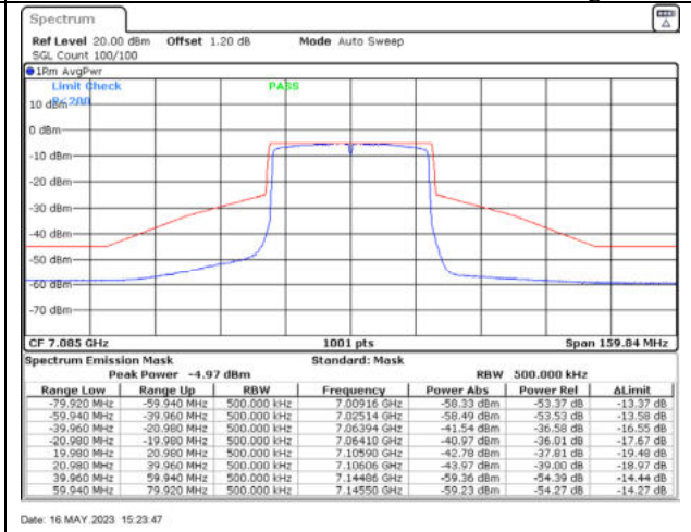
802.11ax40 / 7085MHz / Chain B - Beamforming
