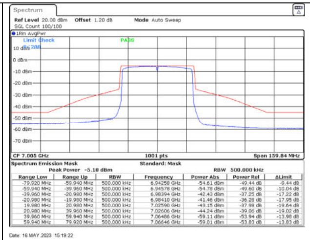
802.11ax40 / 7005MHz / Chain D - Beamforming
