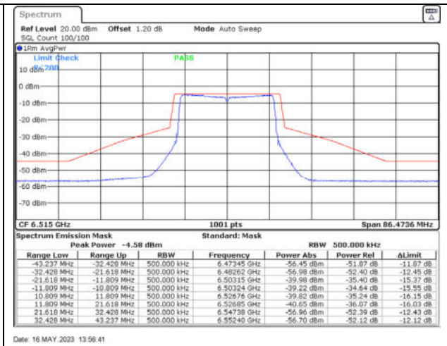
802.11ax20 / 6515MHz / Chain B - Beamforming
