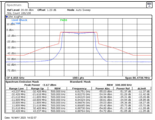
802.11ax20 / 6855MHz / Chain B - Beamforming
