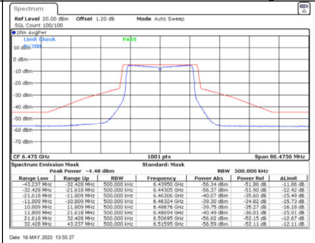
802.11ax20 / 6475MHz / Chain B - Beamforming
