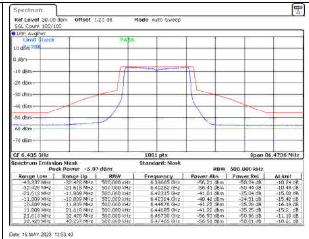
802.11ax20 / 6435MHz / Chain D - Beamforming
