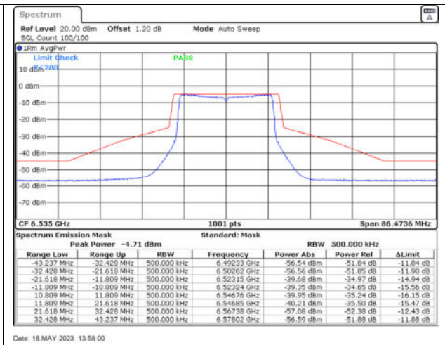
802.11ax20 / 6535MHz / Chain D - Beamforming
