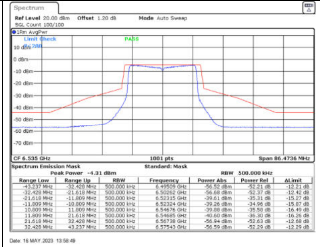
802.11ax20 / 6535MHz / Chain B - Beamforming
