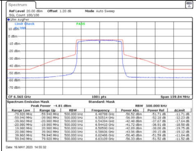
802.11ax40 / 6565MHz / Chain D - Beamforming
