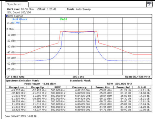
802.11ax20 / 6855MHz / Chain D - Beamforming
