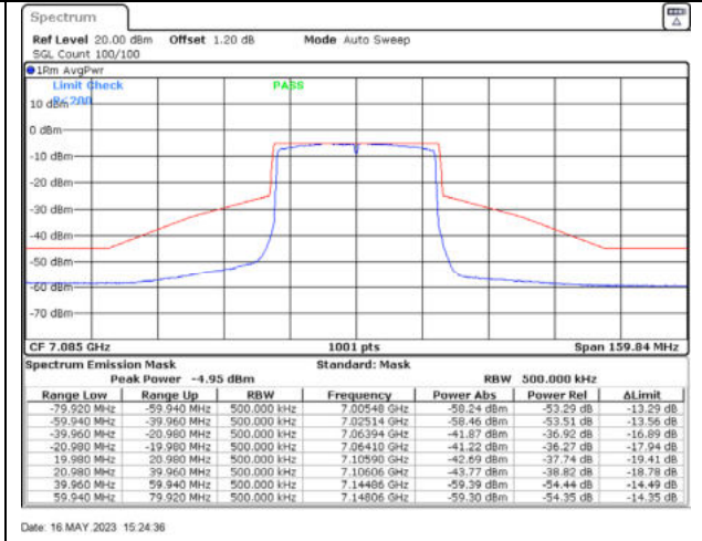
802.11ax40 / 7085MHz / Chain D - Beamforming
