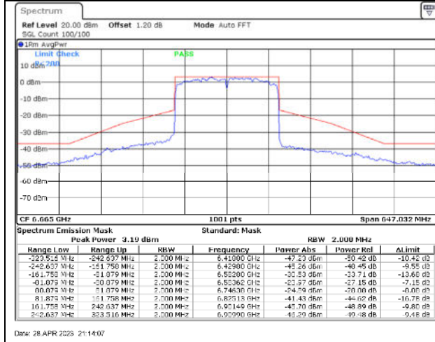
802.11ax160 / 6665MHz / Chain A - CDD
