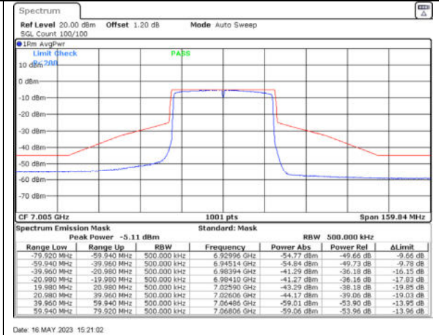
802.11ax40 / 7005MHz / Chain B - Beamforming
