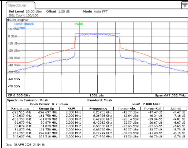
802.11ax160 / 6505MHz / Chain D - CDD
