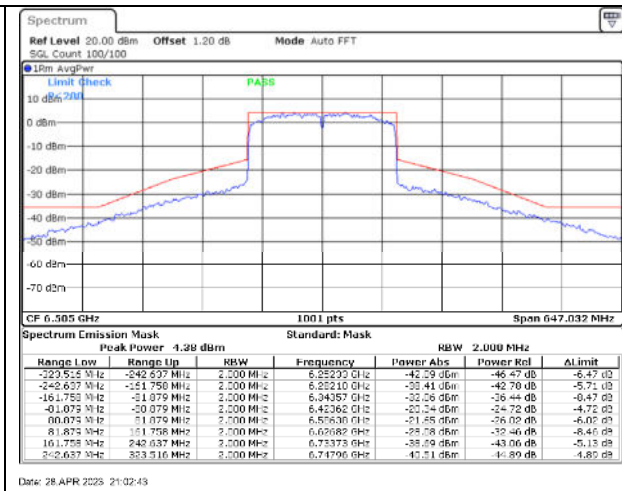
802.11ax160 / 6505MHz / Chain B - CDD
