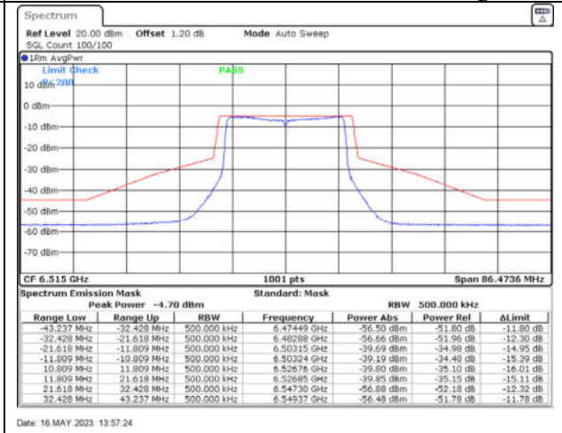
802.11ax20 / 6515MHz / Chain D - Beamforming
