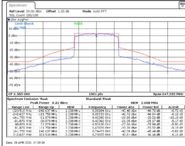
802.11ax160 / 6505MHz / Chain C - CDD
