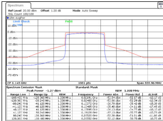
802.11ax80 / 6145MHz / Chain A - Beamforming
