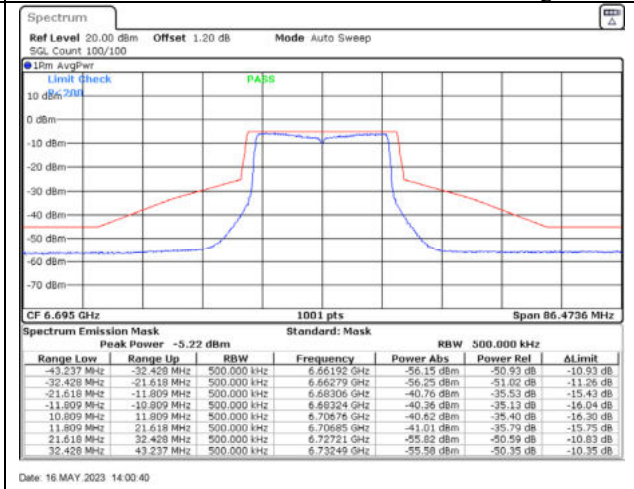
802.11ax20 / 6695MHz / Chain B - Beamforming
