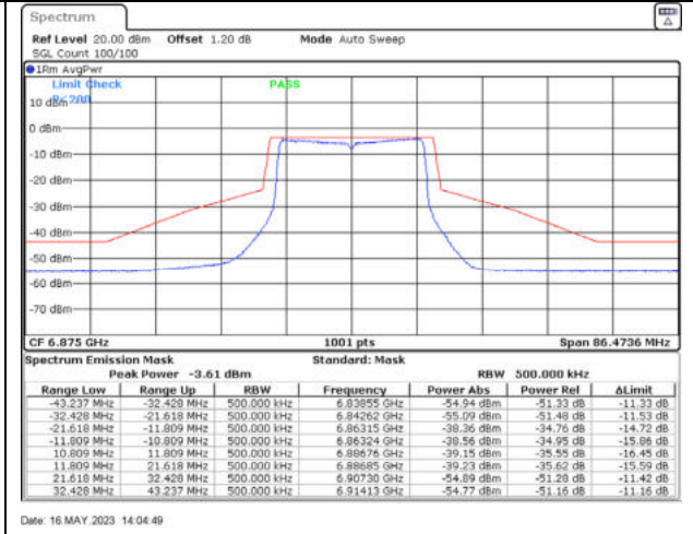
802.11ax20 / 6875MHz / Chain B - Beamforming
