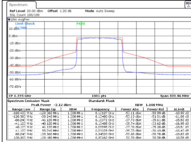
802.11ax80 / 6225MHz / Chain A - Beamforming
