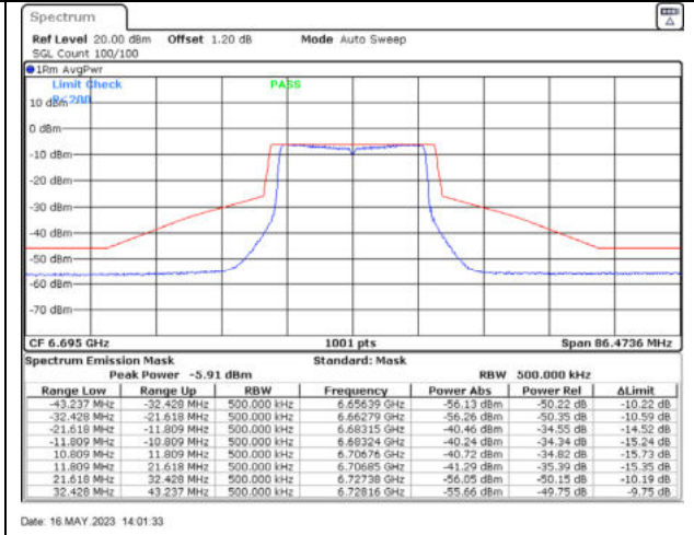
802.11ax20 / 6695MHz / Chain D - Beamforming
