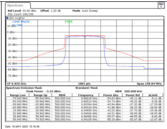
802.11ax40 / 6925MHz / Chain B - Beamforming
