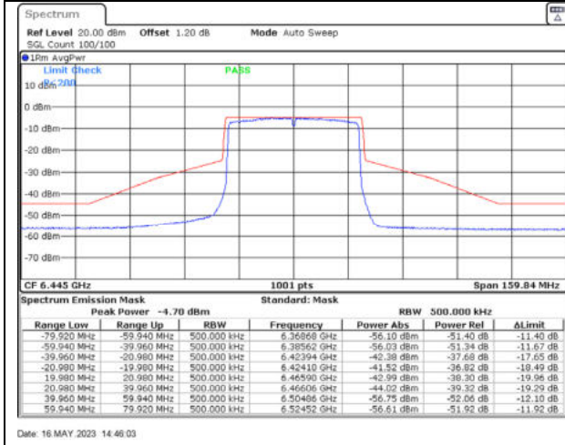
802.11ax40 / 6445MHz / Chain C - Beamforming
