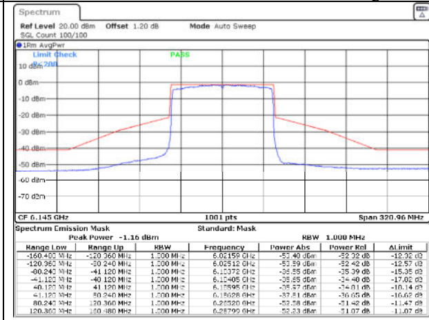
802.11ax80 / 6145MHz / Chain B - Beamforming
