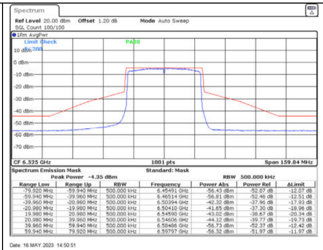
802.11ax40 / 6525MHz / Chain D - Beamforming
