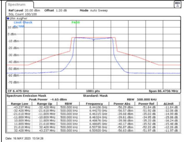
802.11ax20 / 6475MHz / Chain D - Beamforming
