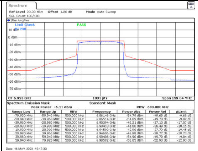
802.11ax40 / 6925MHz / Chain D - Beamforming
