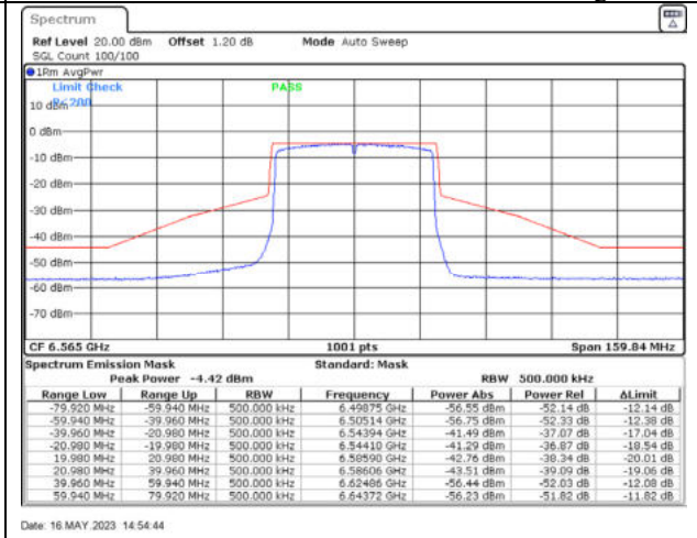
802.11ax40 / 6565MHz / Chain B - Beamforming
