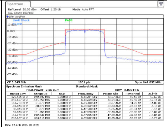
802.11ax160 / 6345MHz / Chain D - CDD
