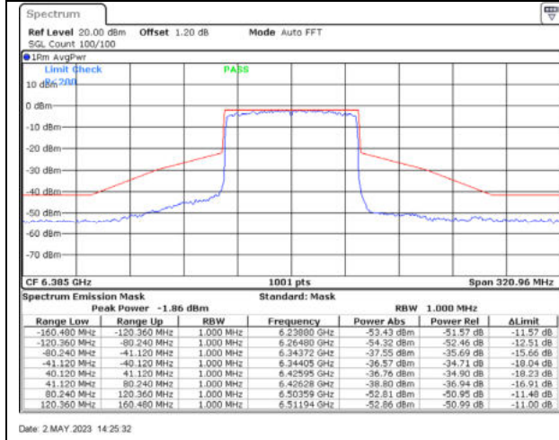
802.11ax80 / 6385MHz / Chain A - CDD
