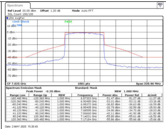
802.11ax80 / 7025MHz / Chain B - CDD
