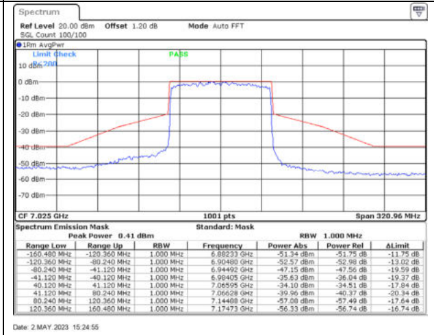
802.11ax80 / 7025MHz / Chain D - CDD
