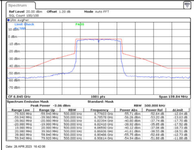
802.11ax40 / 6845MHz / Chain D - CDD
