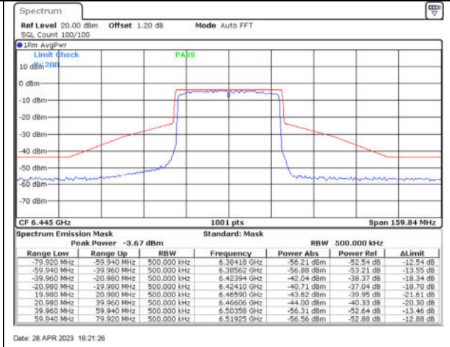
802.11ax40 / 6445MHz / Chain B - CDD
