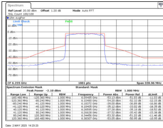
802.11ax80 / 6225MHz / Chain A - CDD
