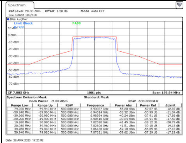
802.11ax40 / 7005MHz / Chain D - CDD
