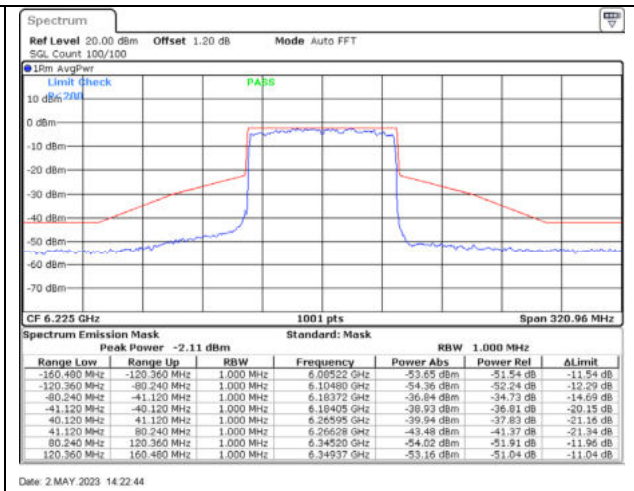
802.11ax80 / 6225MHz / Chain B - CDD
