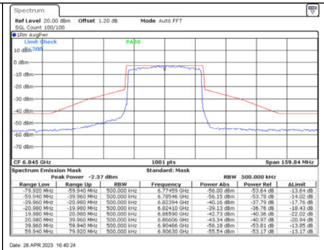
802.11ax40 / 6845MHz / Chain B - CDD
