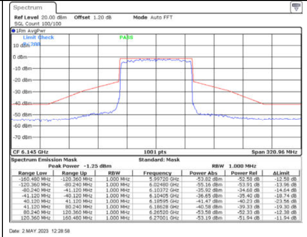
802.11ax80 / 6145MHz / Chain D - CDD
