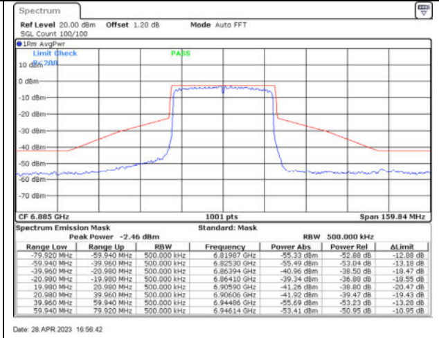
802.11ax40 / 6885MHz / Chain B - CDD
