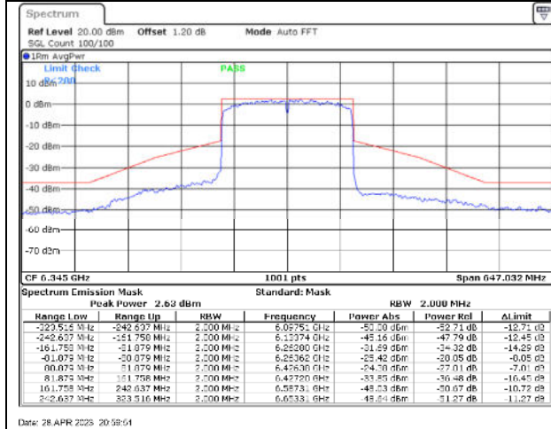
802.11ax160 / 6345MHz / Chain C - CDD
