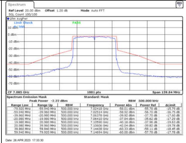
802.11ax40 / 7085MHz / Chain B - CDD
