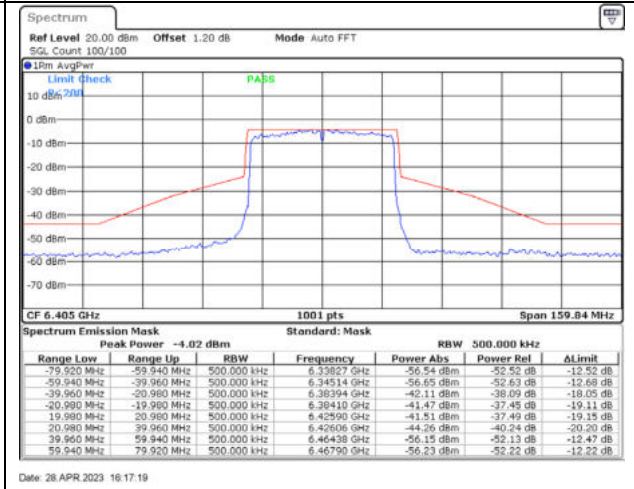
802.11ax40 / 6405MHz / Chain D - CDD
