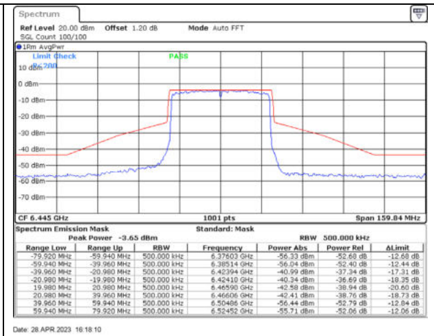
802.11ax40 / 6445MHz / Chain D - CDD
