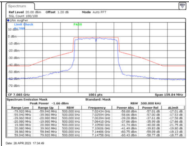
802.11ax40 / 7085MHz / Chain D - CDD
