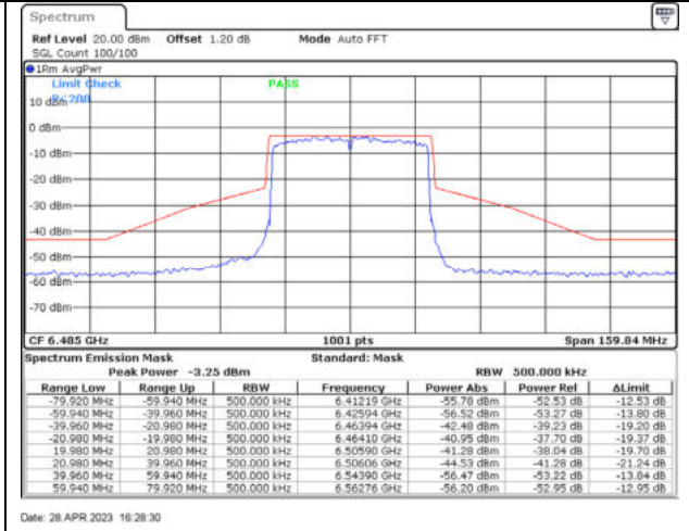
802.11ax40 / 6485MHz / Chain D - CDD
