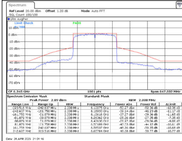
802.11ax160 / 6345MHz / Chain A - CDD
