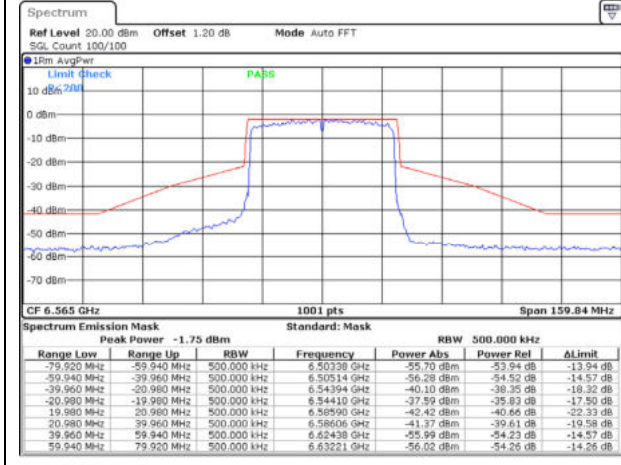
802.11ax40 / 6565MHz / Chain B - CDD
