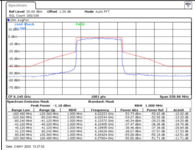
802.11ax80 / 6145MHz / Chain B - CDD
