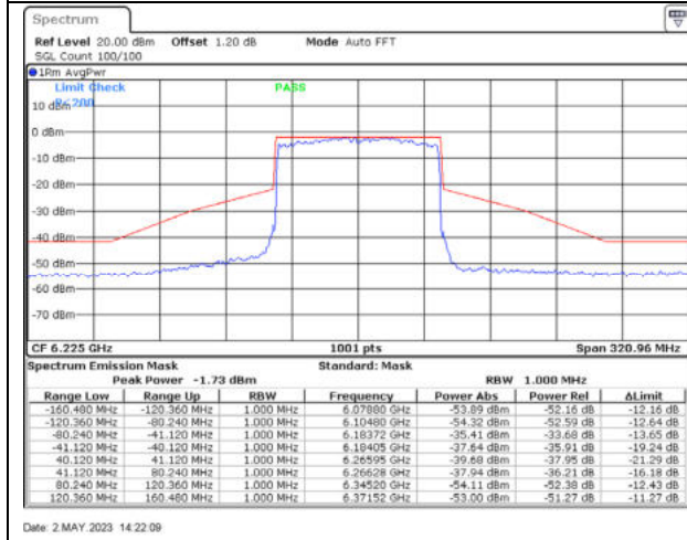
802.11ax80 / 6225MHz / Chain C - CDD
