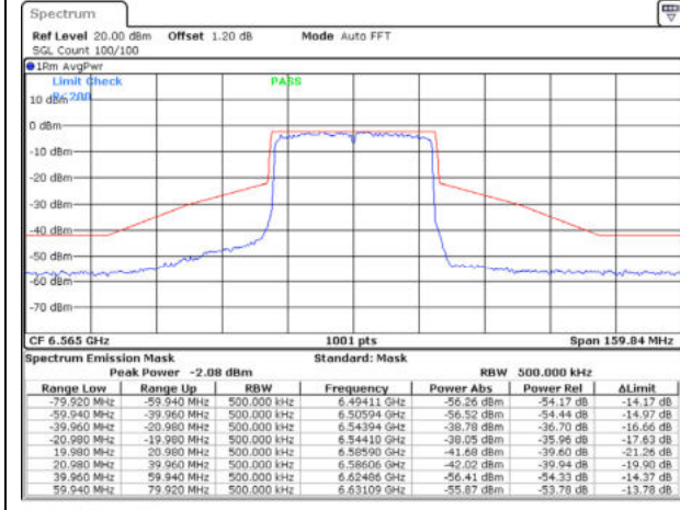
802.11ax40 / 6565MHz / Chain A - CDD
