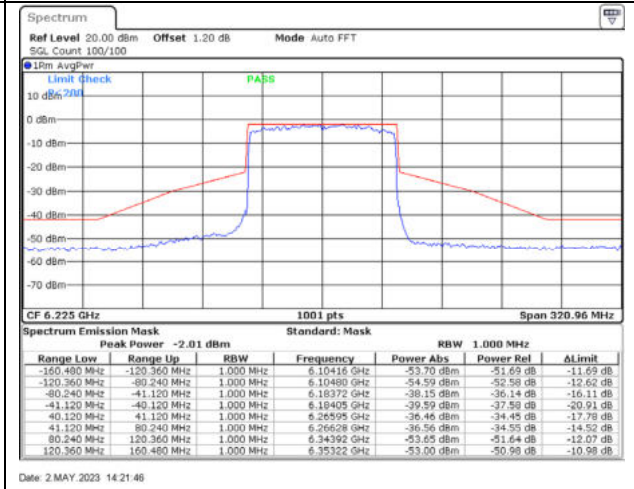
802.11ax80 / 6225MHz / Chain D - CDD
