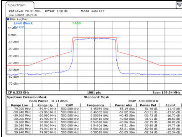
802.11ax40 / 6525MHz / Chain A - CDD
