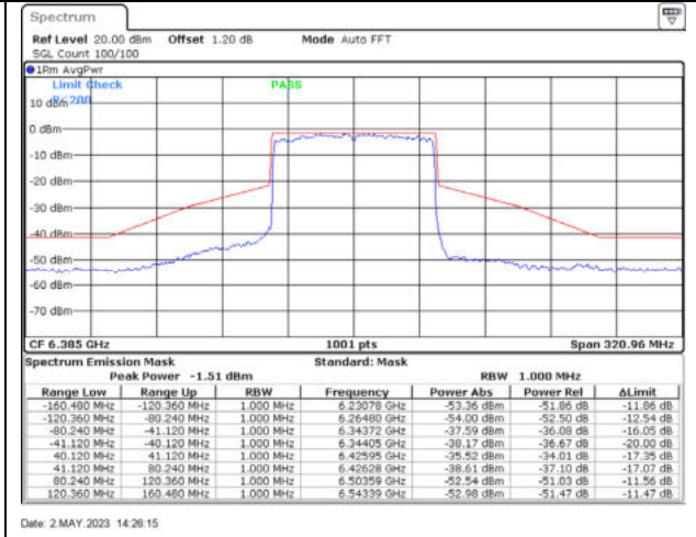
802.11ax80 / 6385MHz / Chain B - CDD
