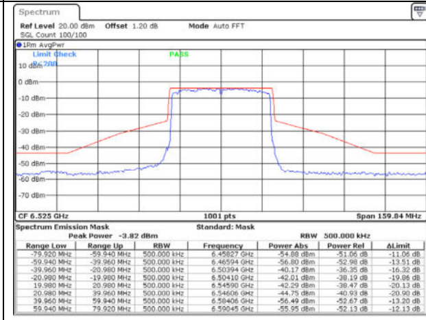
802.11ax40 / 6525MHz / Chain B - CDD
