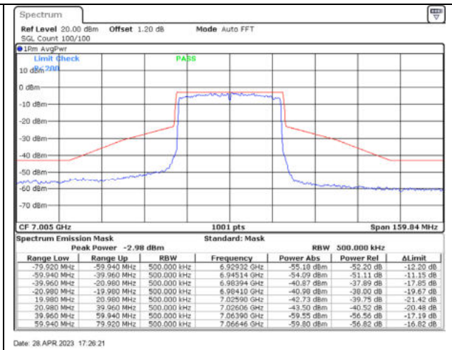
802.11ax40 / 7005MHz / Chain B - CDD
