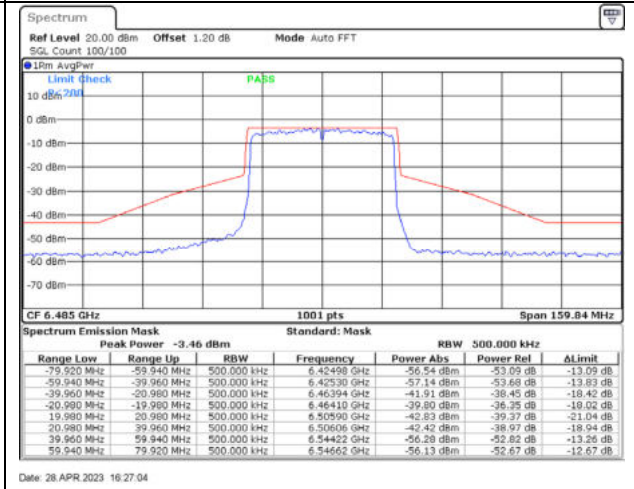
802.11ax40 / 6485MHz / Chain B - CDD
