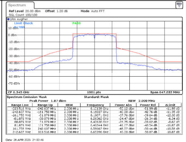
802.11ax160 / 6345MHz / Chain B - CDD
