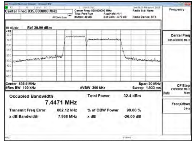
LTE CA Band 5B_256-QAM_CH20416+CH20455_3M+5M_15RB0+25RB0
