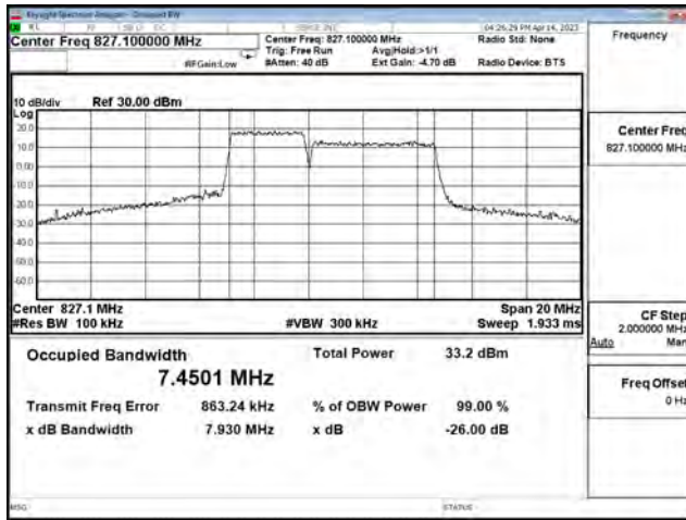
LTE CA Band 5B_64-QAM_CH20586+CH20625_3M+5M_15RB0+25RB0
