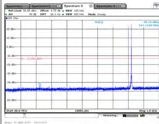
LTE Band 5_CH20450_10M_1RB0_QPSK_Below 1GHz
