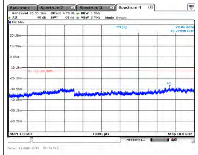
LTE CA Band 5B_CH20501+CH20540_3M+5M_QPSK_1RB14+1RB0_Above 1GHz
