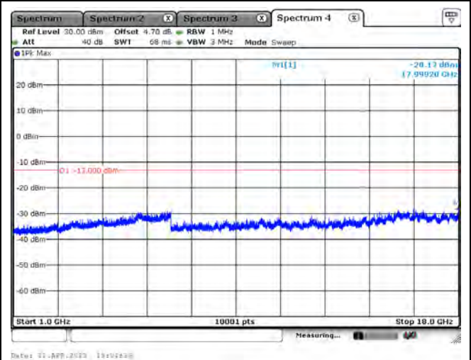
LTE Band 5_CH20525_10M_1RB0_QPSK_Above 1GHz
