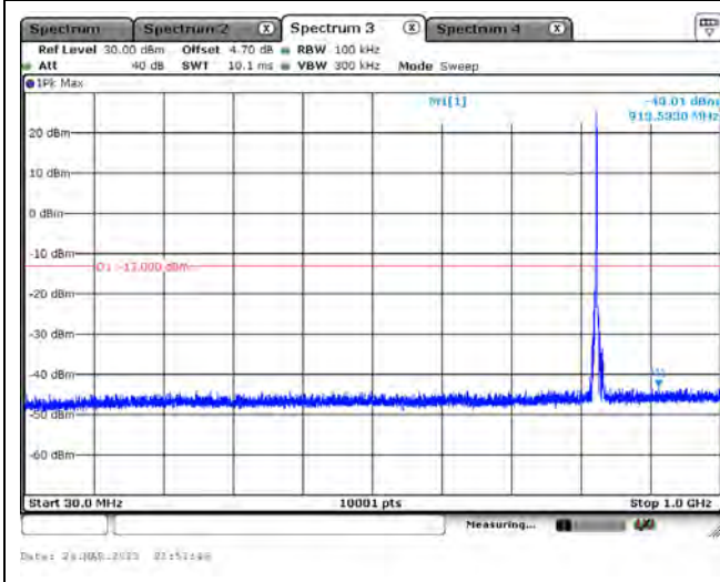
LTE CA Band 5B_CH20501+CH20540_3M+5M_QPSK_1RB14+1RB0_Below 1GHz
