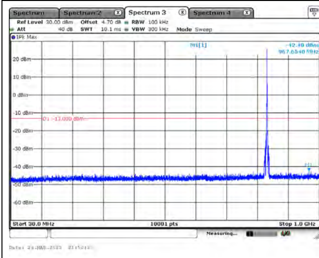
LTE CA Band 5B_CH20586+CH20625_3M+5M_QPSK_1RB14+1RB0_Below 1GHz
