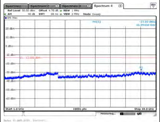
LTE Band 5_CH20450_10M_1RB0_QPSK_Above 1GHz
