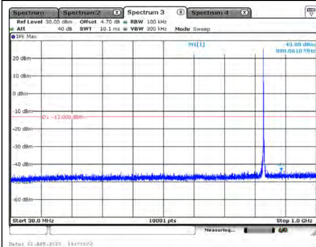
LTE Band 5_CH20525_10M_1RB0_QPSK_Below 1GHz
