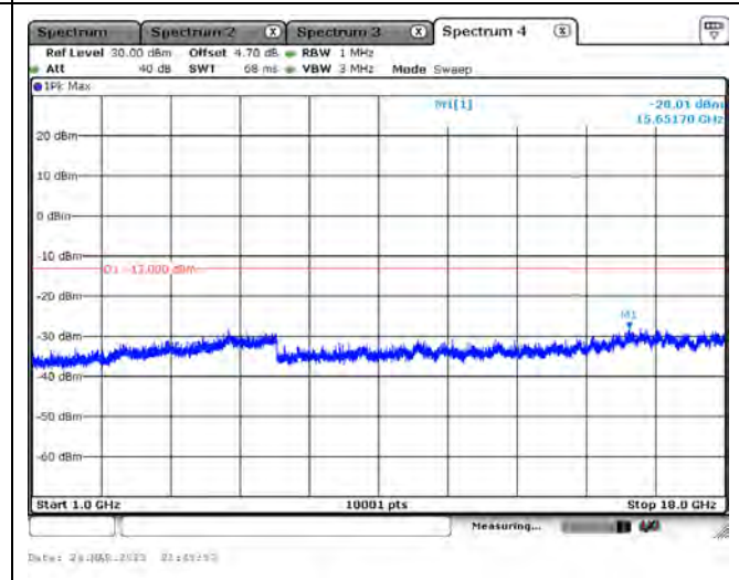
LTE CA Band 5B_CH20586+CH20625_3M+5M_QPSK_1RB14+1RB0_Above 1GHz
