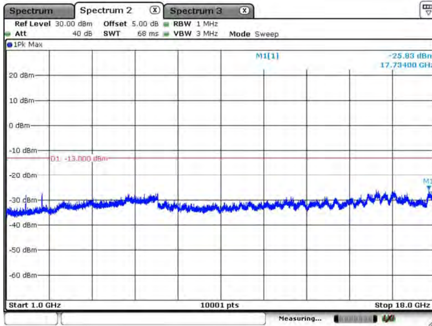
B12_CH23017_1.4M_1RB0_QPSK_Above 1G
