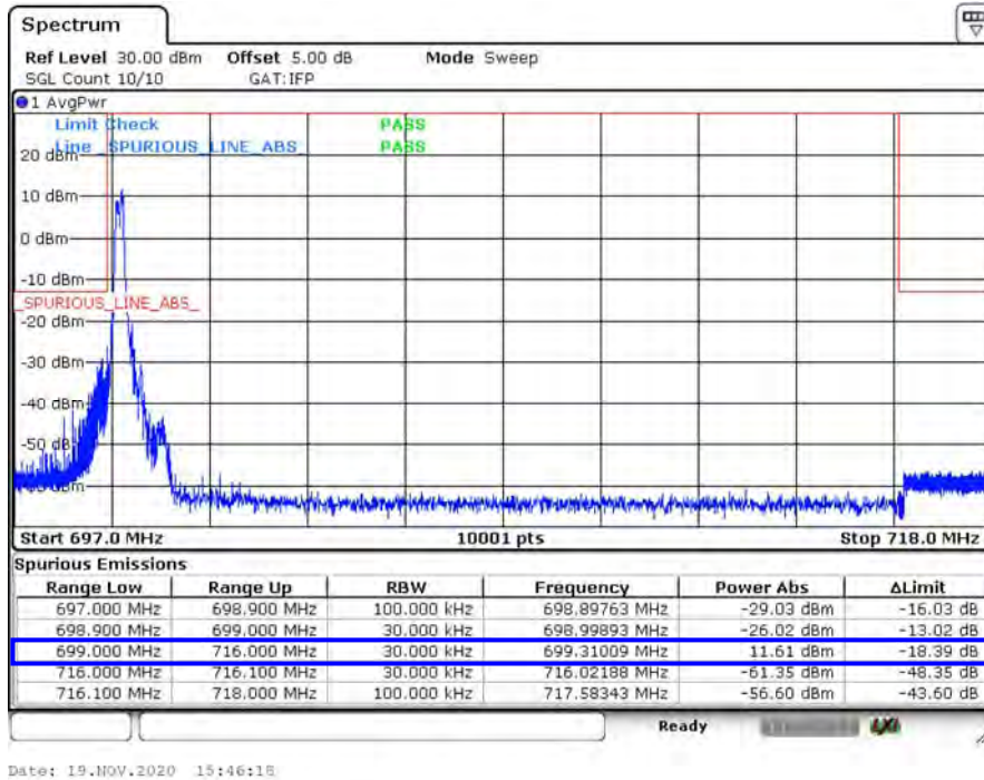
LTE_B12_CH23017_1.4M_QPSK_1RB0
