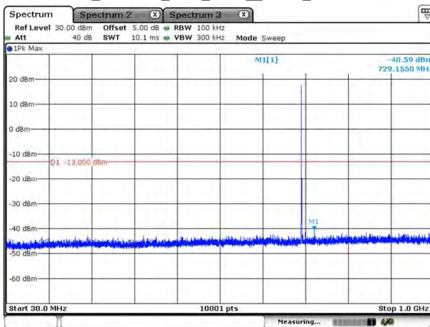
B12_CH23017_1.4M_1RB0_QPSK_Below 1G
