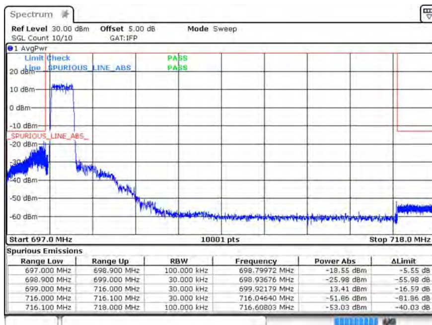
LTE_B12_CH23017_1.4M_QPSK_6RB0
