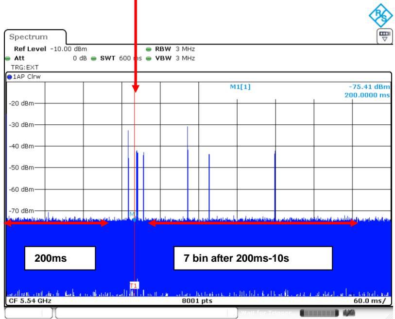
Zoom-in 600 ms Timing Plot
