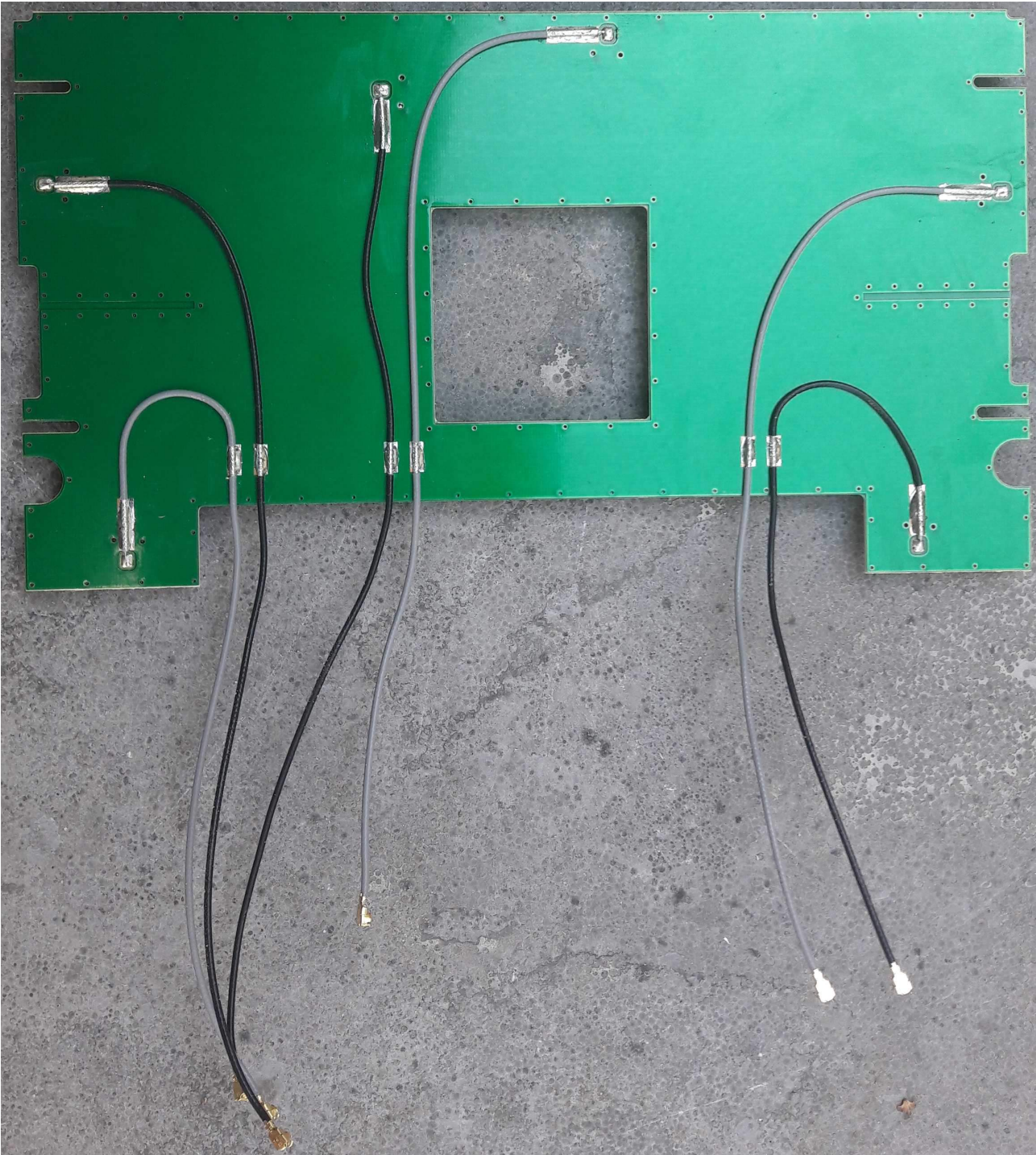
Antenna – backside view
