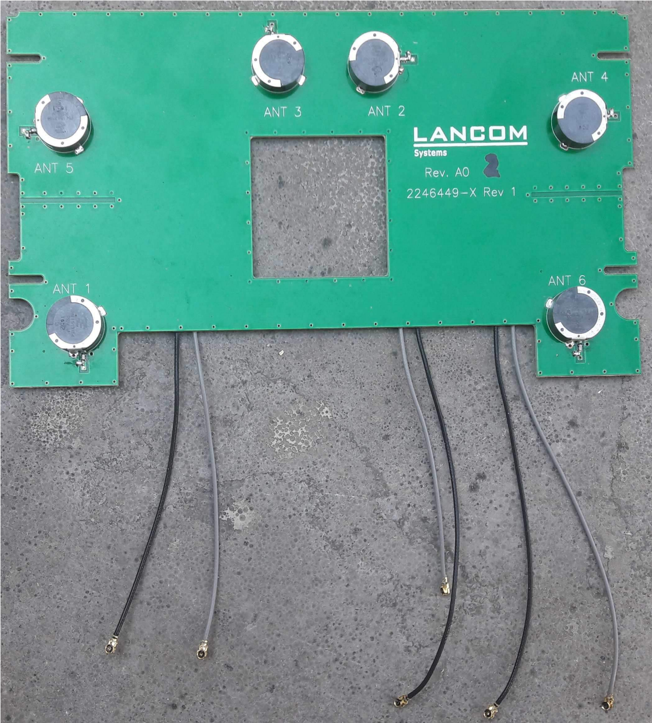
Antenna – front view
