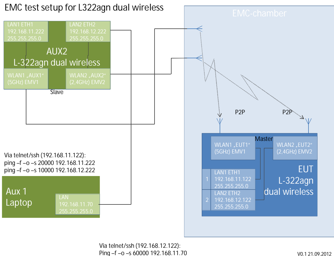
Figure 1 Test Setup for colocation tests
