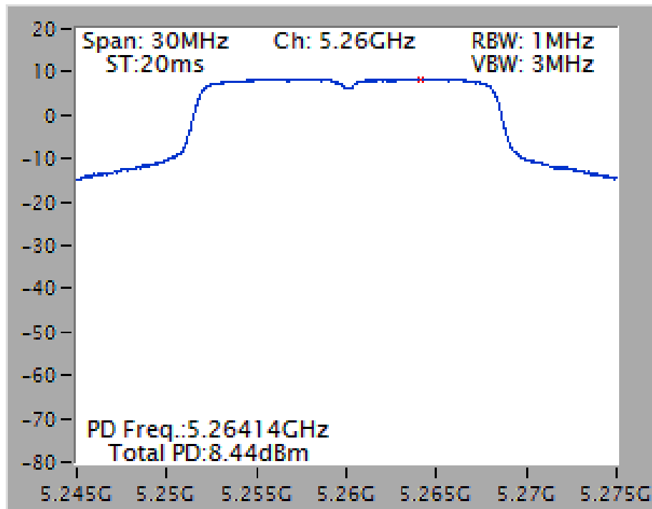
Power Density Plot on Configuration IEEE 802.11a / Chain 1 + Chain 2 / 5260 MHz
