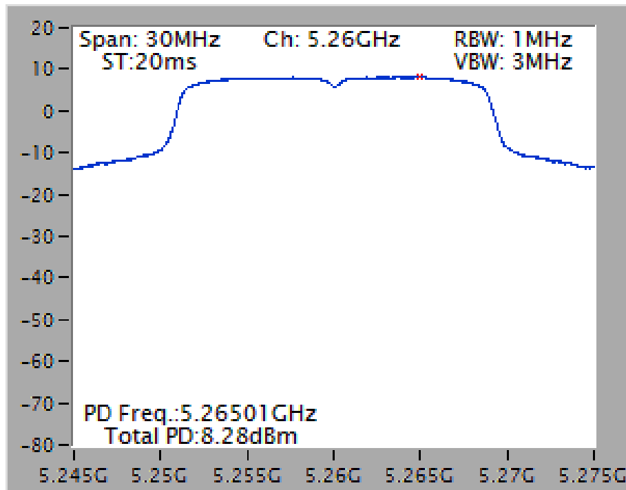
Power Density Plot on Configuration IEEE 802.11n MCS0 20MHz / Chain 1 + Chain 2 / 5260 MHz
