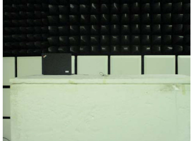
Part_15_407_WLAN_5G_Radiated_Setup
