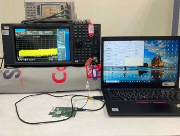
Part_15_407_WLAN_5G_Conducted_Setup
