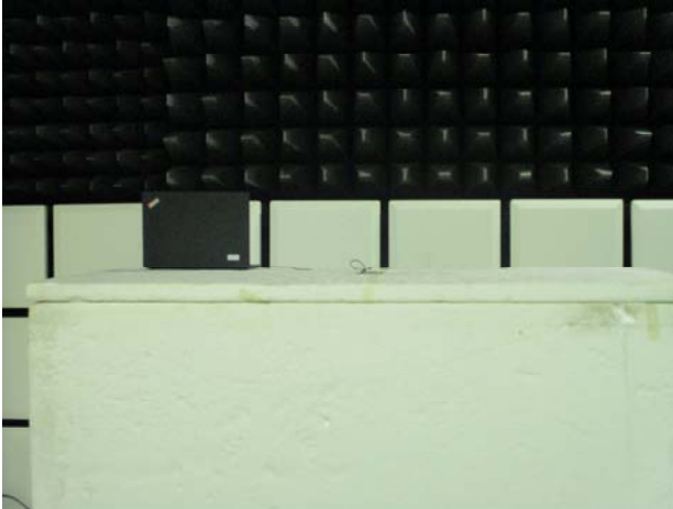
Part_15_247_WLAN_2.4G_Radiated_Setup
