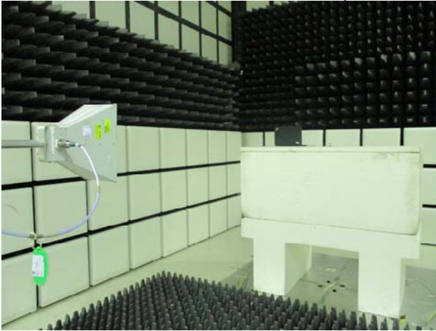
Part_15_407_WLAN_5G_Radiated_Setup
