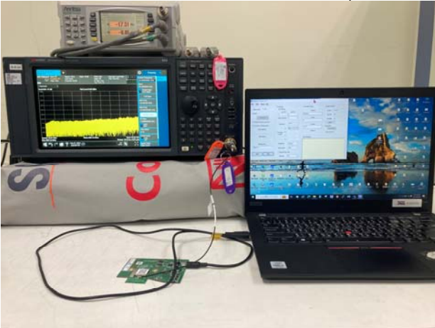
Part_15_407_WLAN_5G_Conducted_Setup
