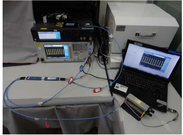
Part_15_407_WLAN_5G_Normal_DFS_Setup
