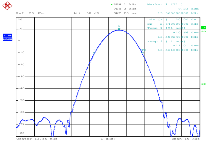
20 dB / 99% Bandwidth Plot on 13.56 MHz
