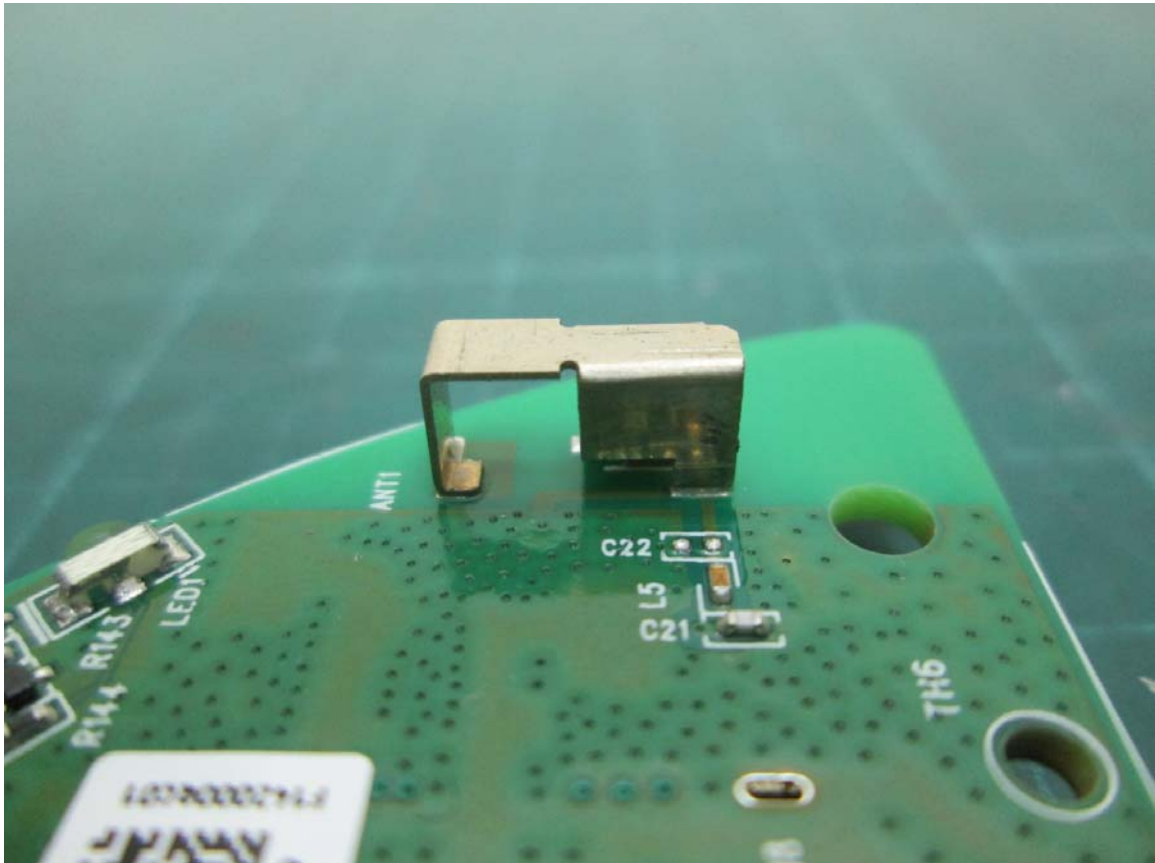
Zigbee Antenna
