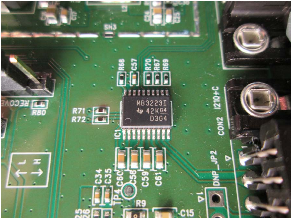
Interface board
