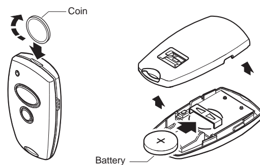
Figure 2. Battery Compartment
