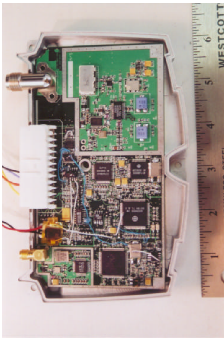
NJIL0CA01 - Top Removed
