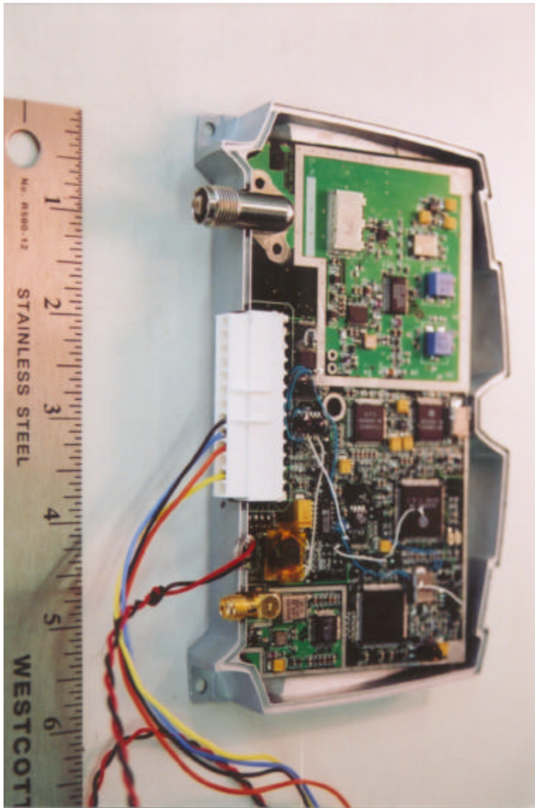
NJILOCA01 - Top Removed Angled
