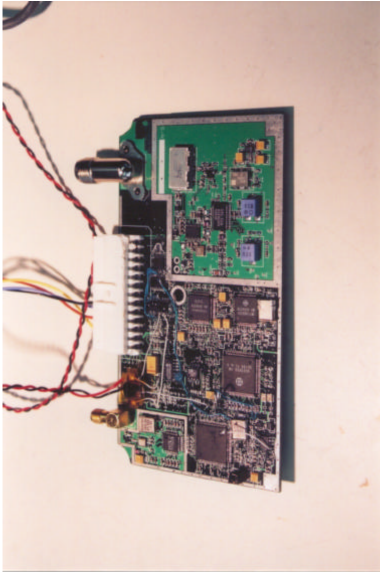
NJILOCA01 - Top of CCA Angled from Rear
