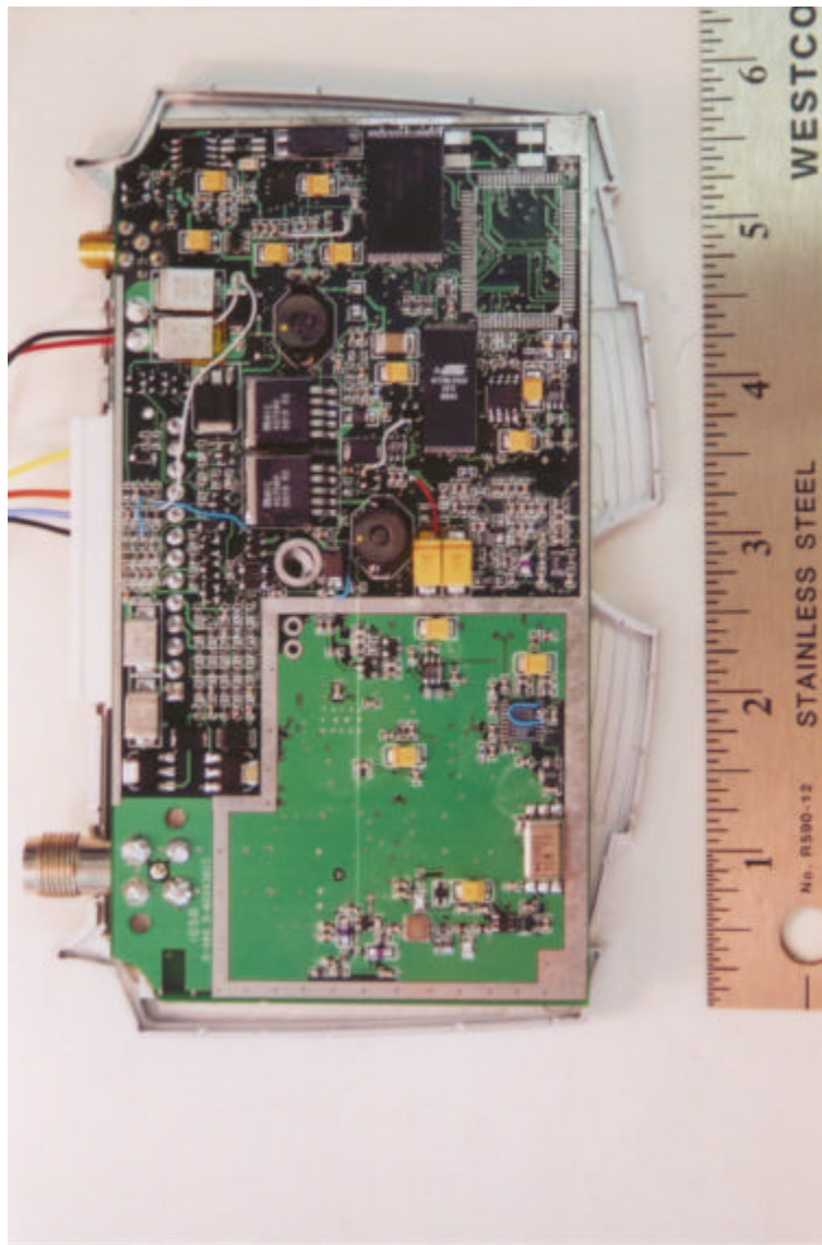
NJILOCA01 - Bottom Removed
