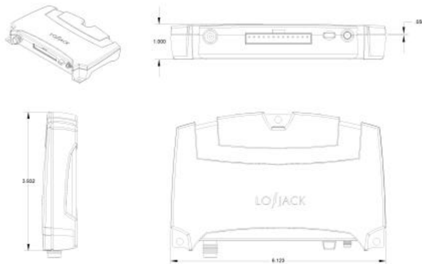
LoCate-001 housing
