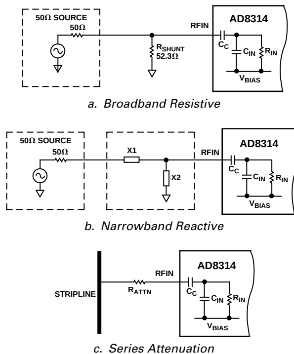
Figure 32. Input Coupling Options
