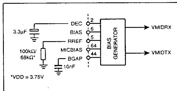
Fig. 16 Bias Circuits
