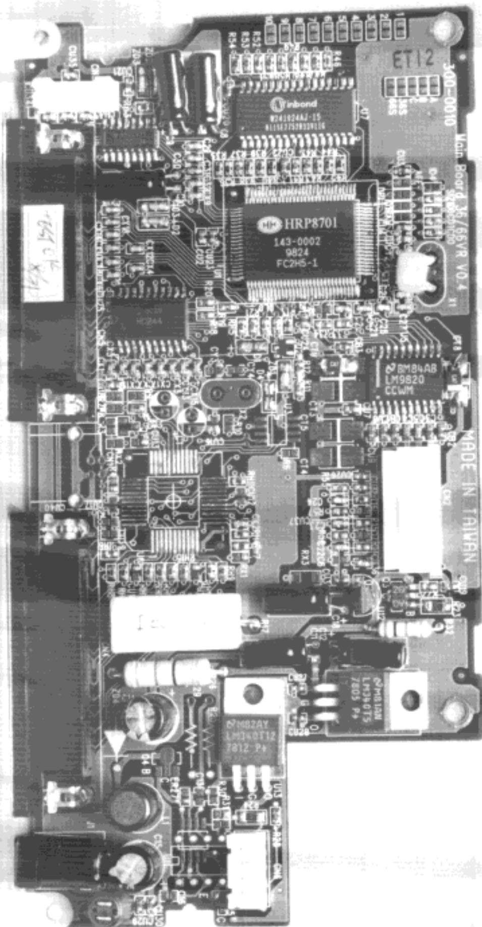
Photograph of EUT Construction Main Board for (Model: DP66V-I03 & 0275-011)
