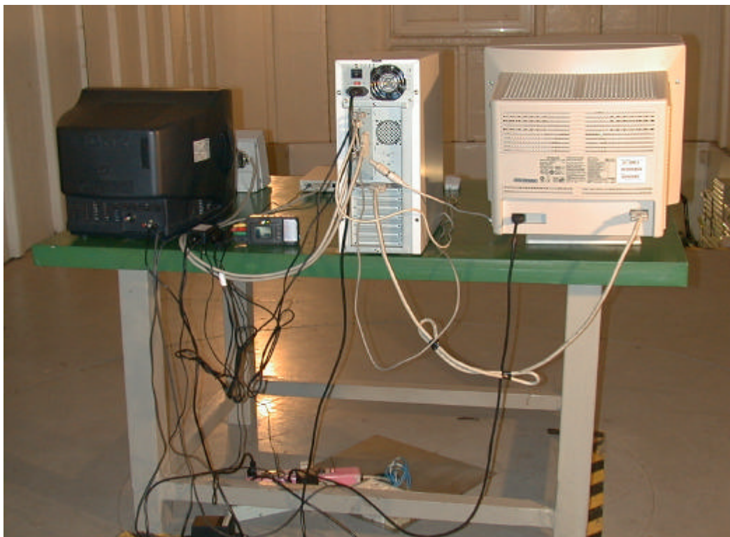
Back View of Radiated Test (Mode 2)
