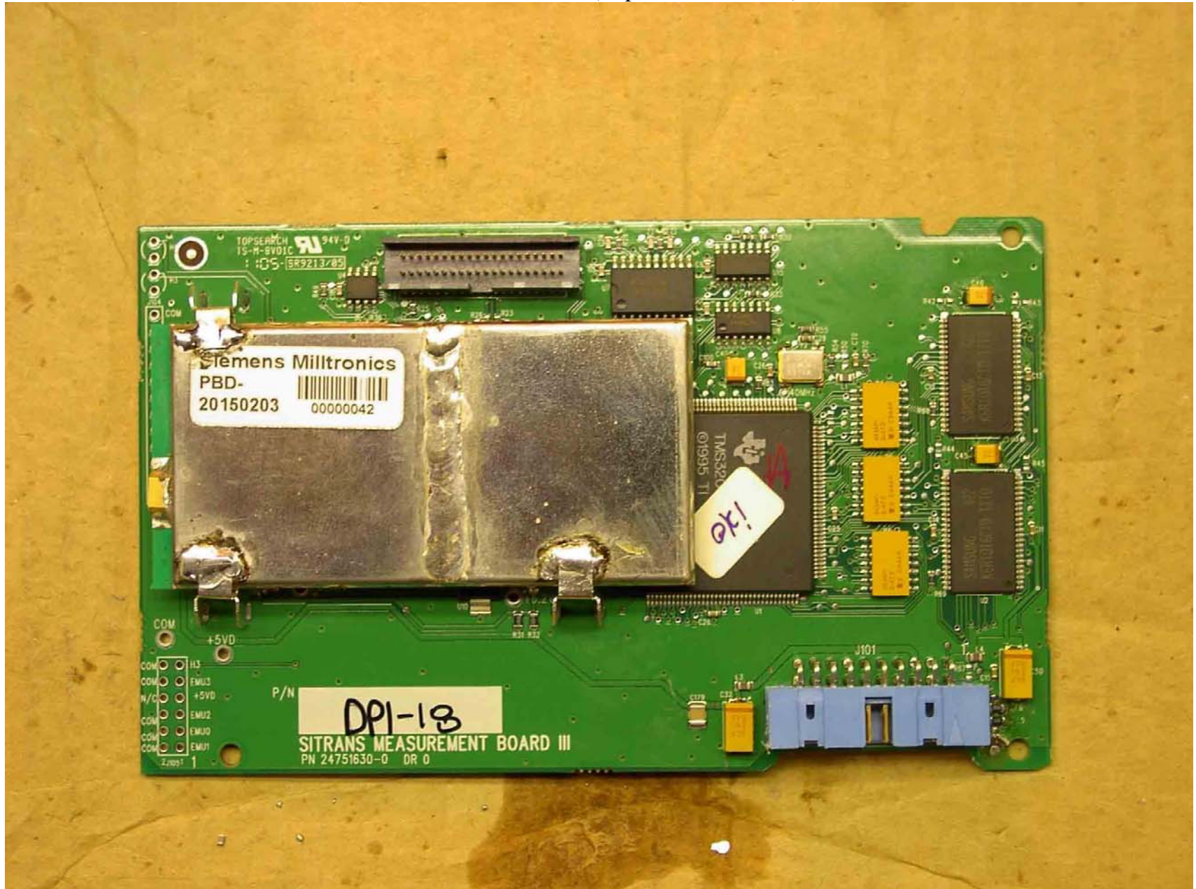
Measurement Board (Top with Shield Can)
