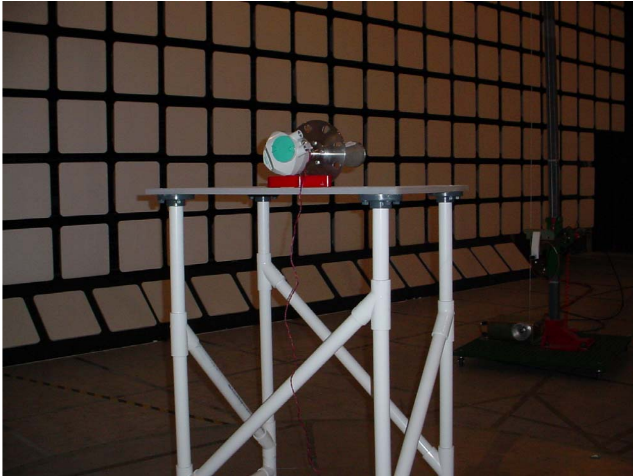
Plot #4: Radiated Emissions below 1 GHz from SITRANS LR 260
