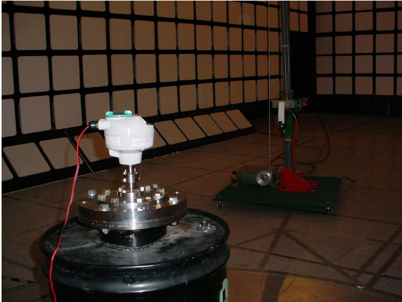
Plot #6: Radiated Emissions from SITRANS LR 260 mounted on top of the metal tank
