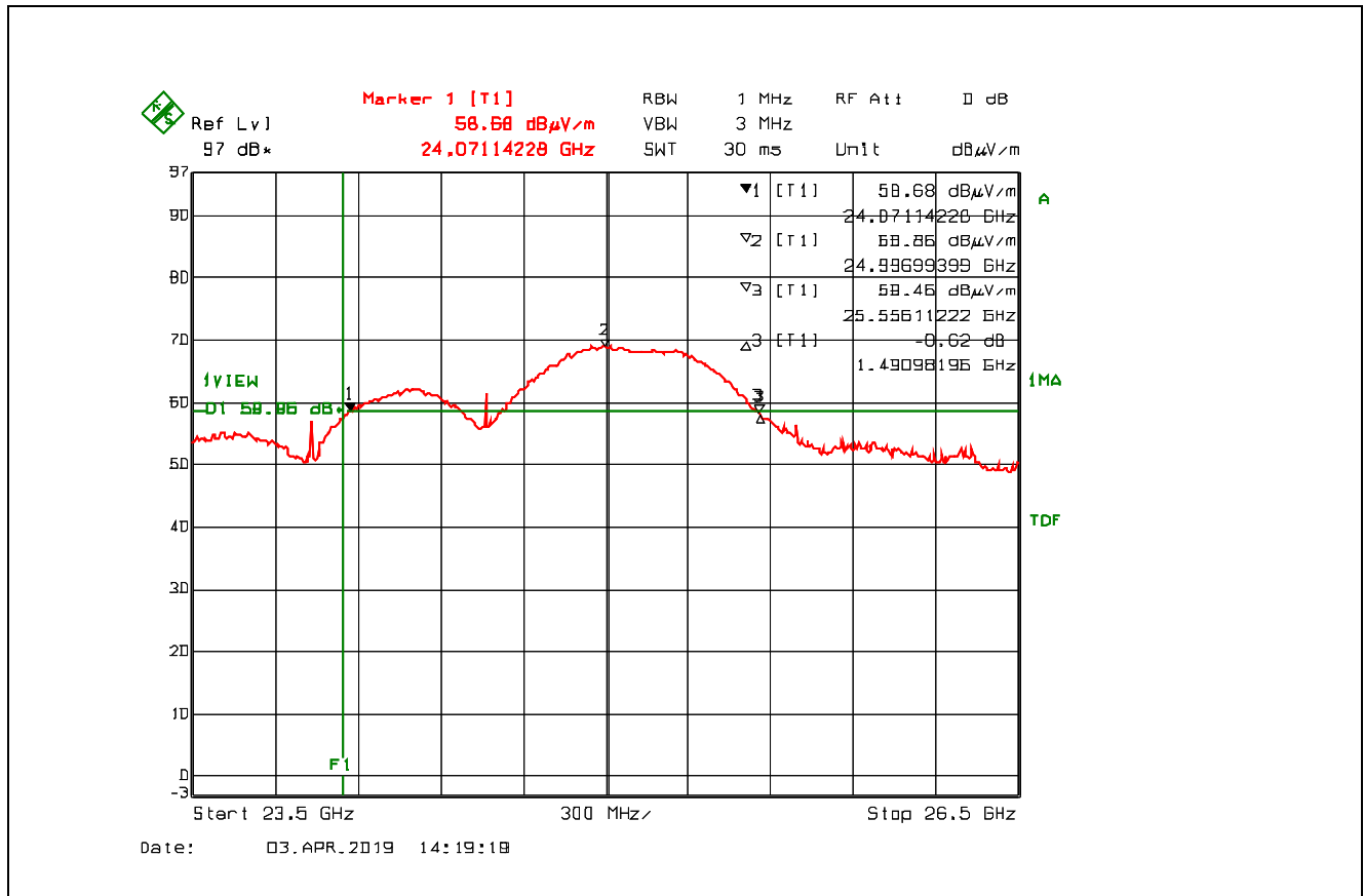
Plot 5.2.3.1. 10 dB Bandwidth, Fc: 25.1 GHz- Vertical
