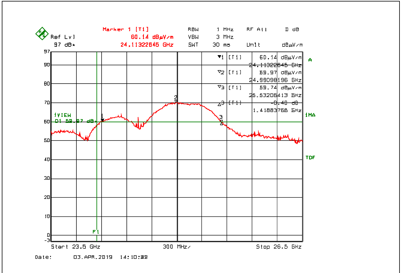
Plot 5.2.3.2. 10 dB Bandwidth, Fc: 25.1 GHz - Horizontal
