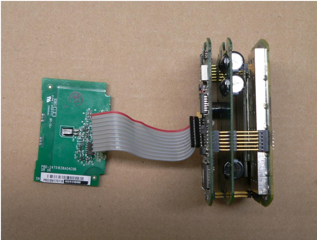
1.4 Board stack opposite long side
