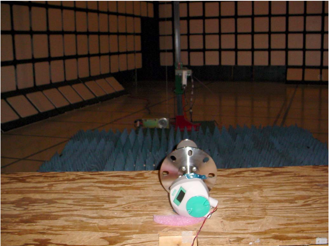
Radiated Emissions at 3 m Distance (above 1 GHz)
