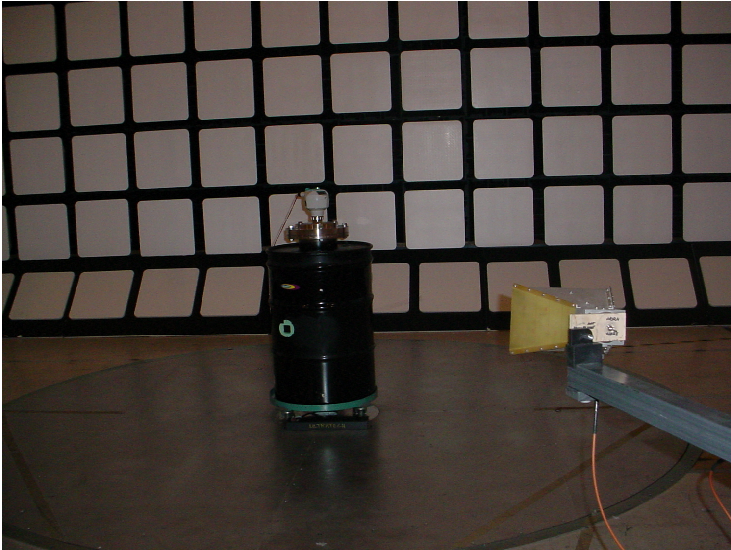
Plot #6: Radiated Emissions from SITRANS LR 250 mounted on top of the metal tank
