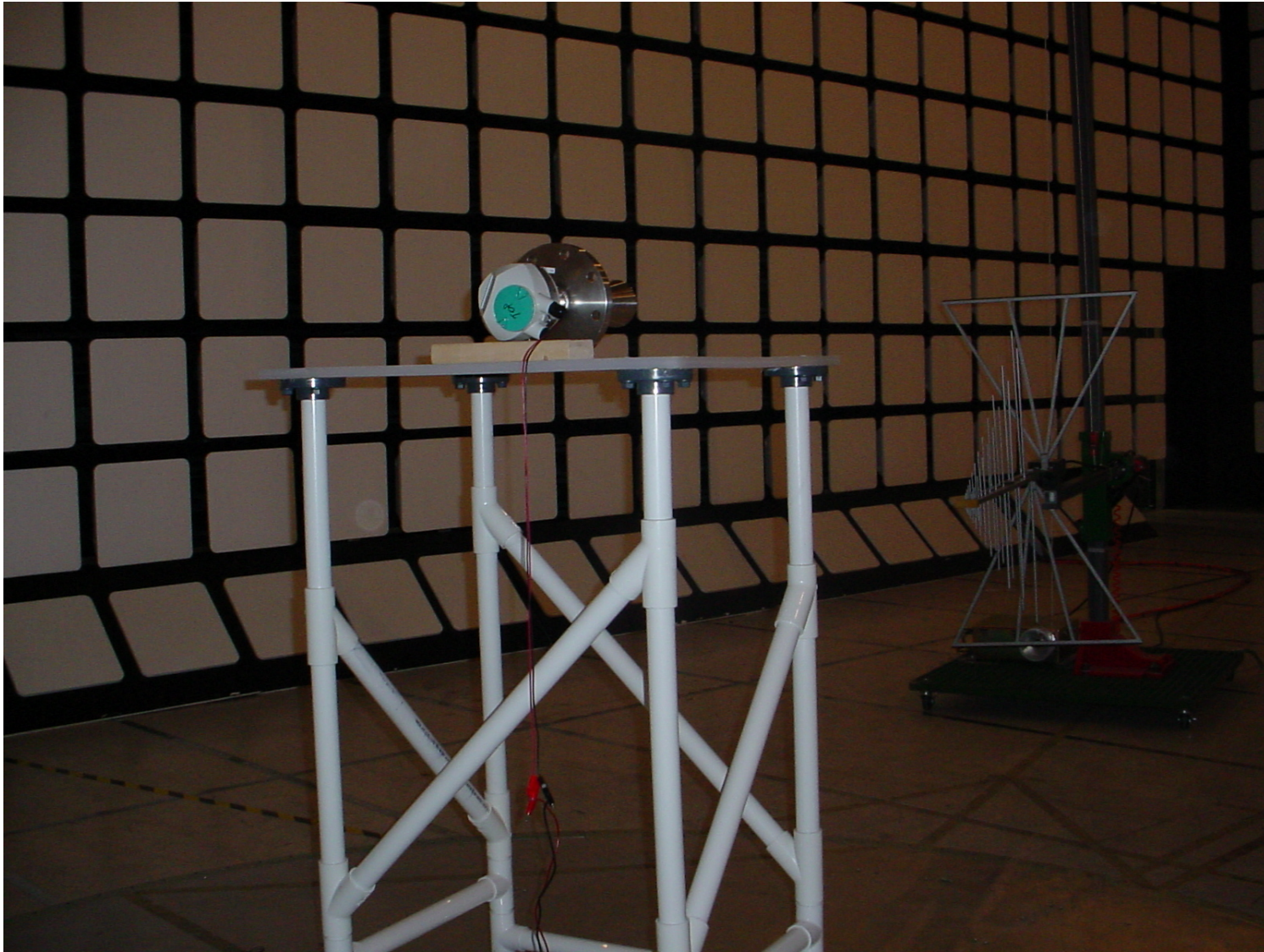
Plot #4: Radiated Emissions below 1 GHz from SITRANS LR 250
