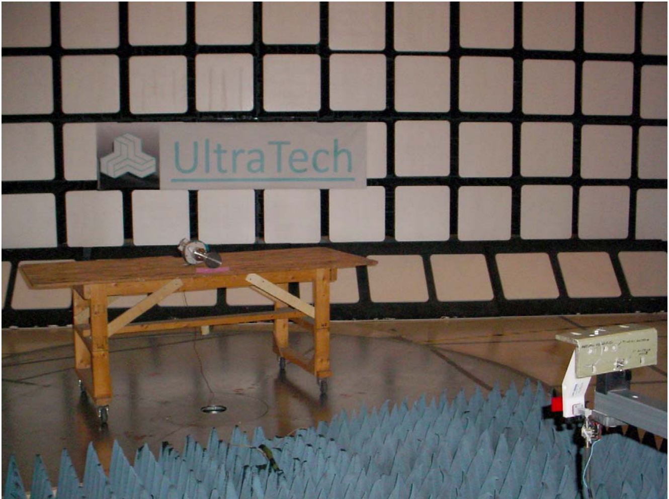
Radiated Emissions at 3 m Distance (rear view)
