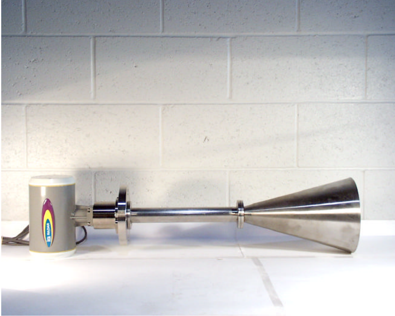
PICTURE #2: MILLTRONICS IQ RADAR160 WITH 4" HORN ANTENNA & ANTENNA EXTENSION
