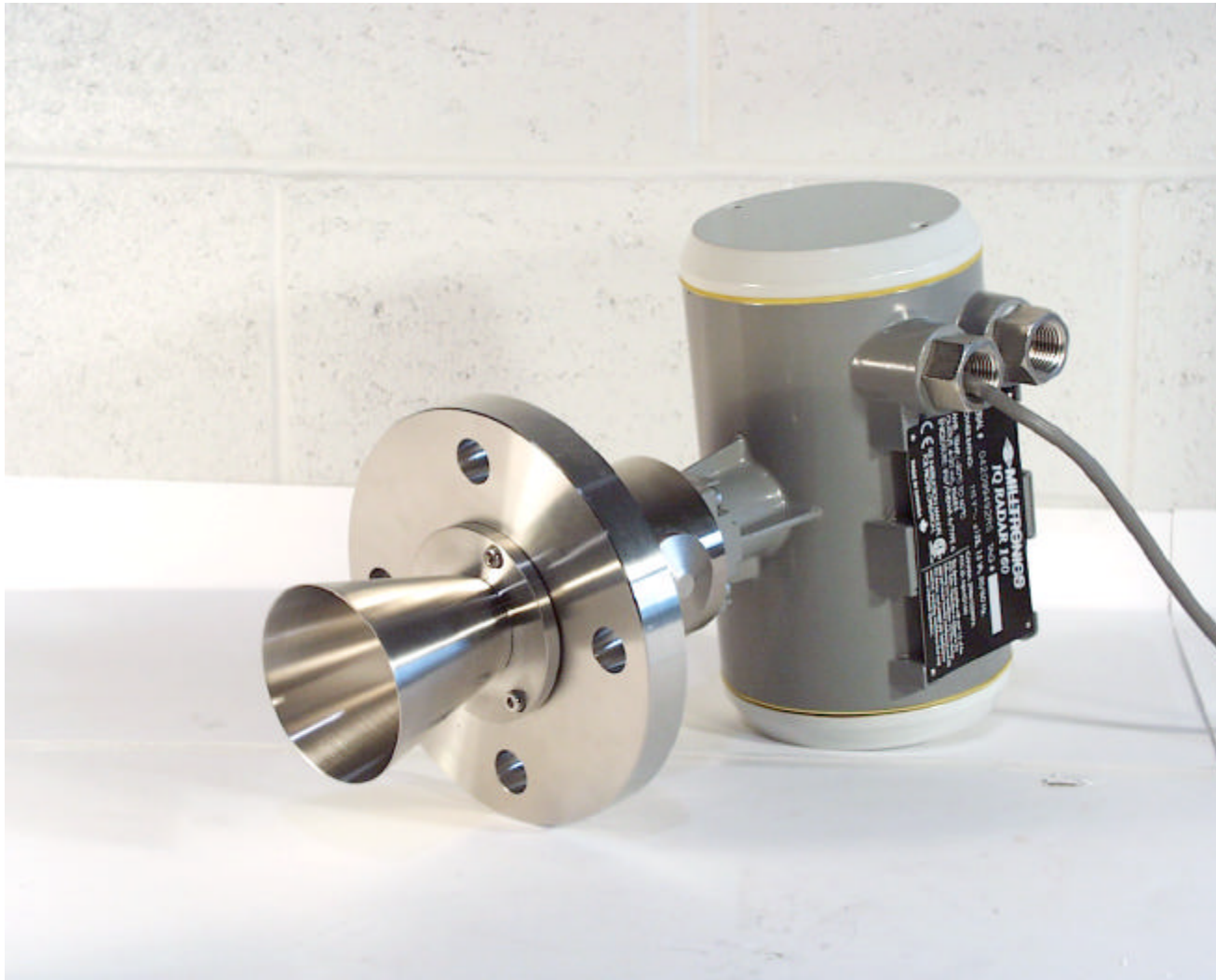
PICTURE #1: MILLTRONICS IQ RADAR160 WITH 3" HORN ANTENNA, NO ANTENNA EXTENSION
