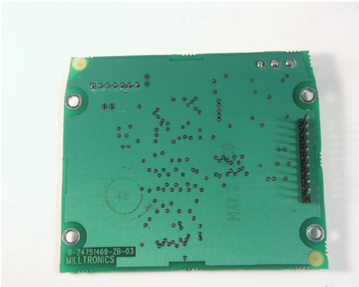
MILLTRONICS IQ-RADAR 160
