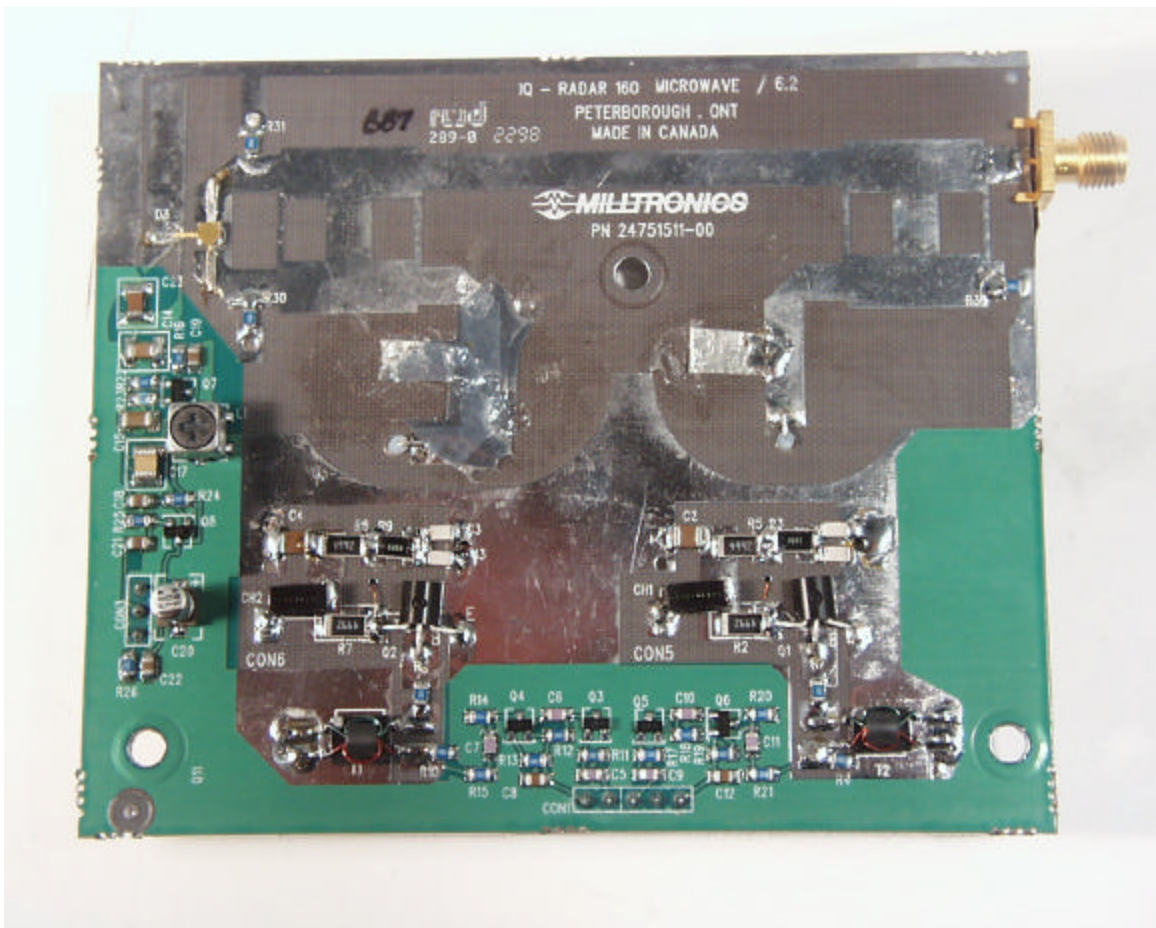
MILLTRONICS IQ-RADAR 160 - RADIO PRINTED CIRCUIT BOARD
