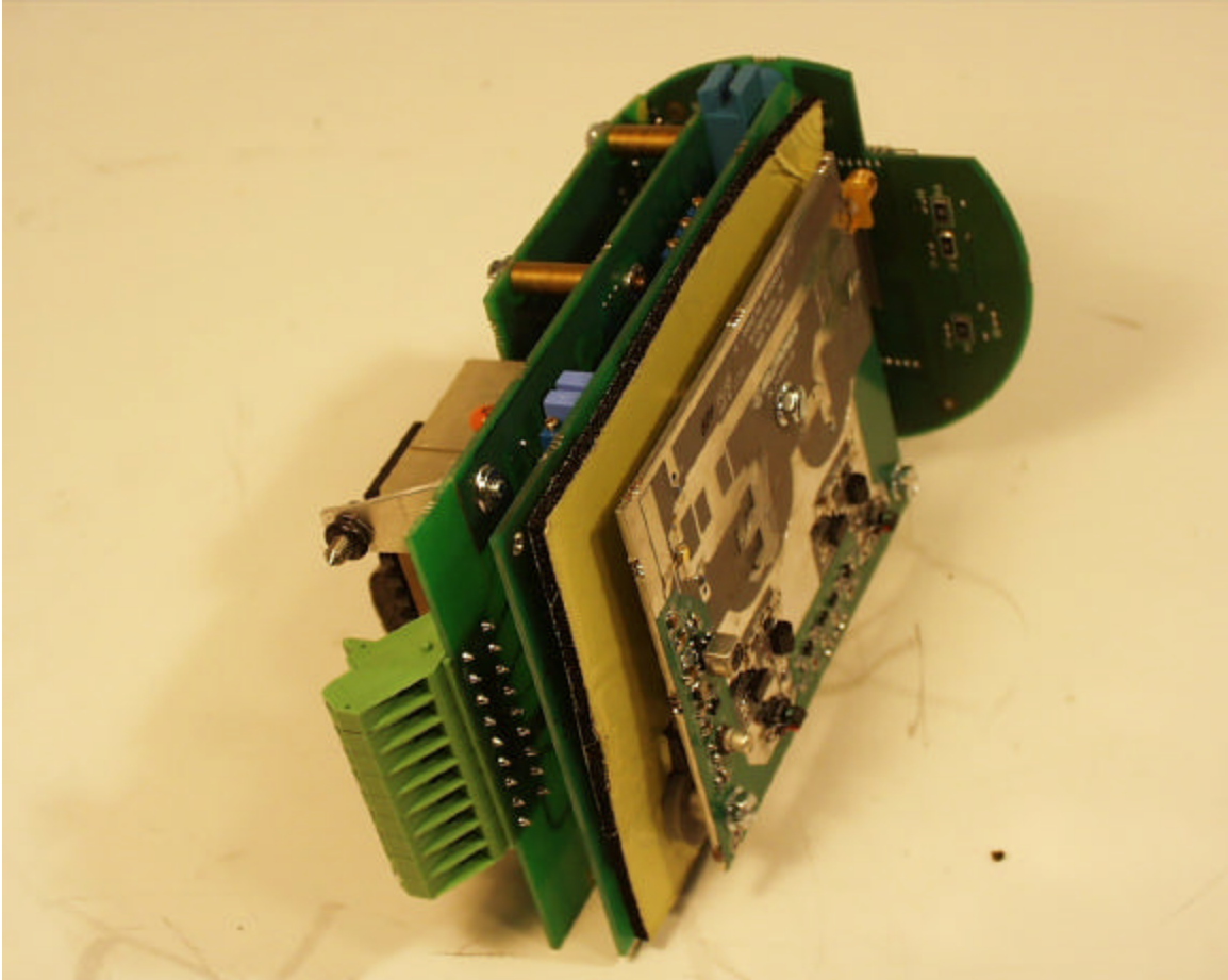
MILLTRONICS IQ-RADAR 160
