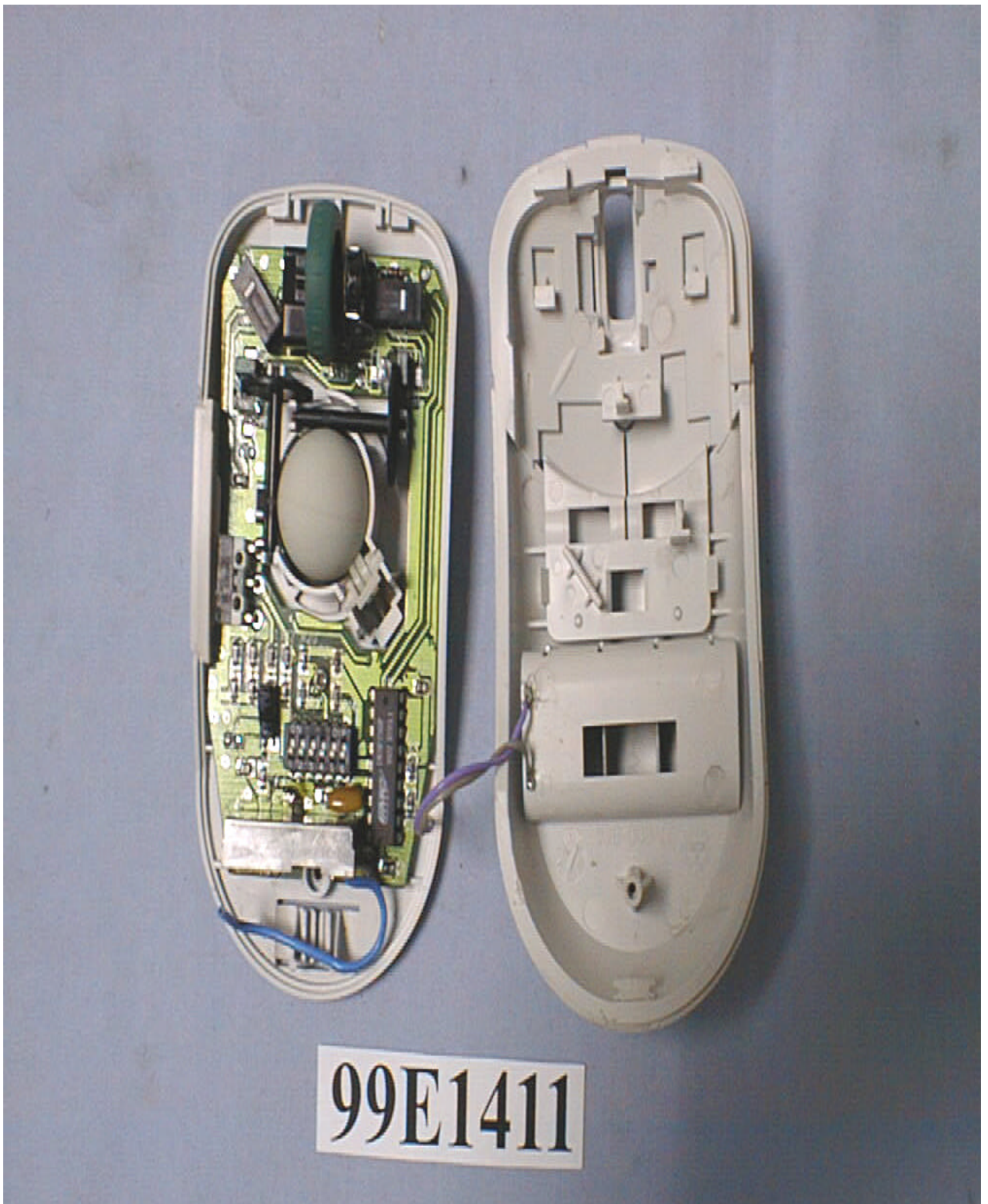
Photo # 4 Unit Partially Disassembled
