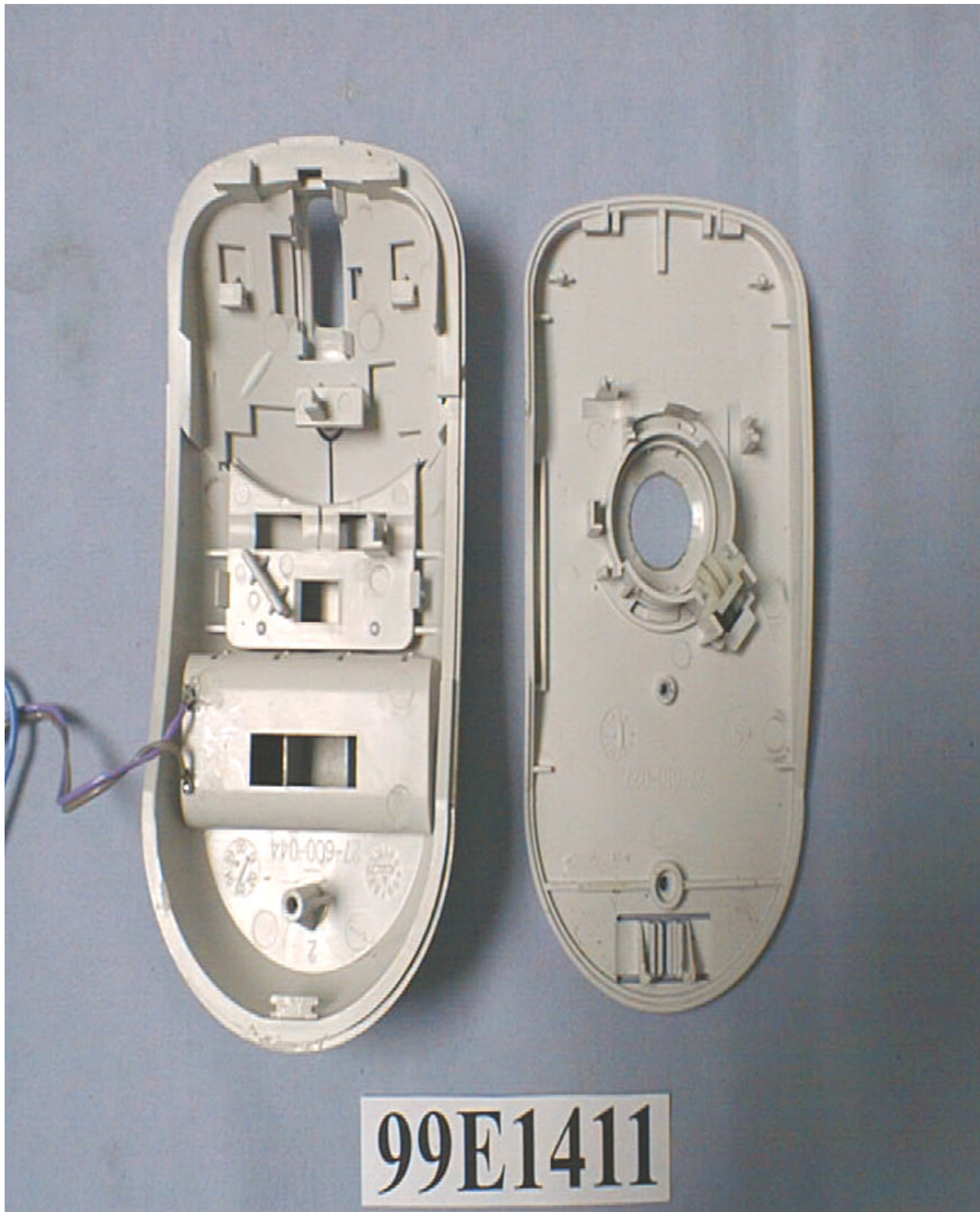
Photo # 7 Unit Partially Disassembled
