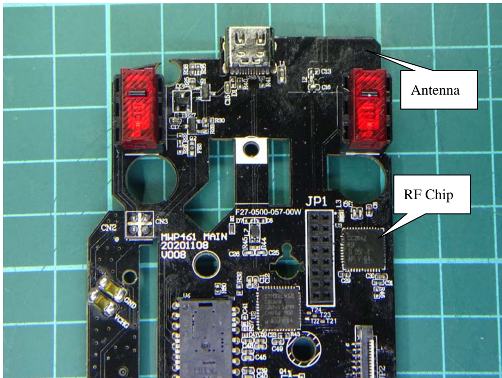
(23) EUT Photo
