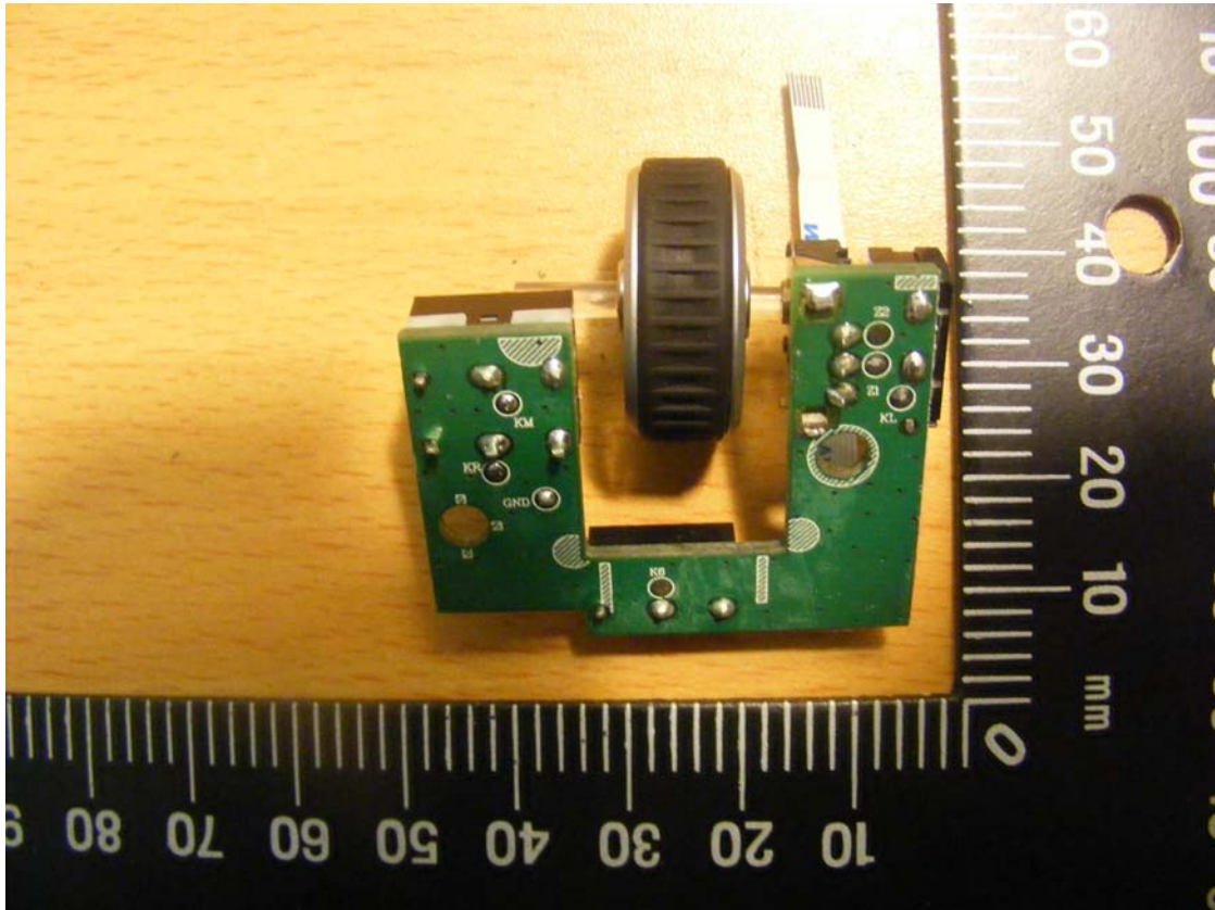
09 Rear view of Main board 3
