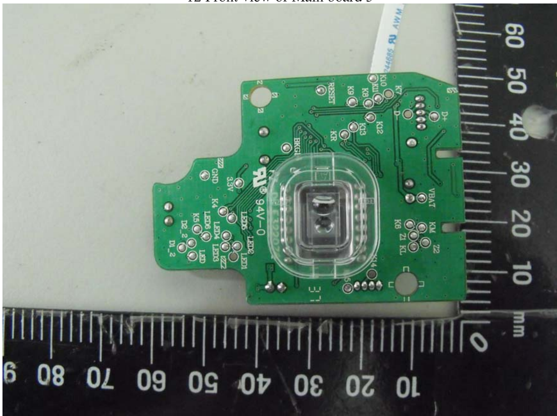
12 Front view of Main board 5
