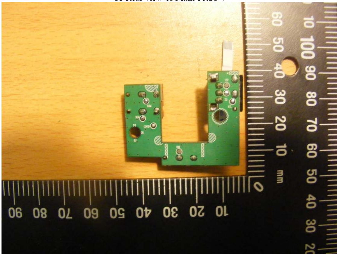
11 Rear view of Main board 4
