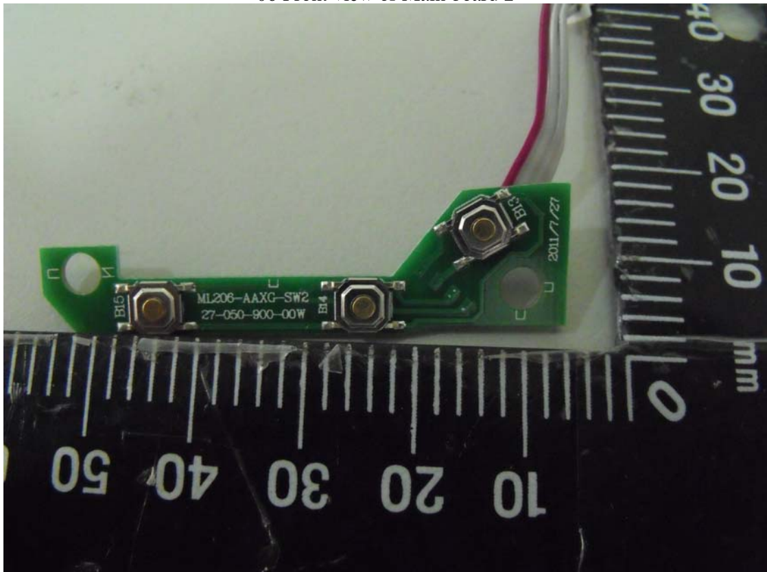
06 Front view of Main board 2
