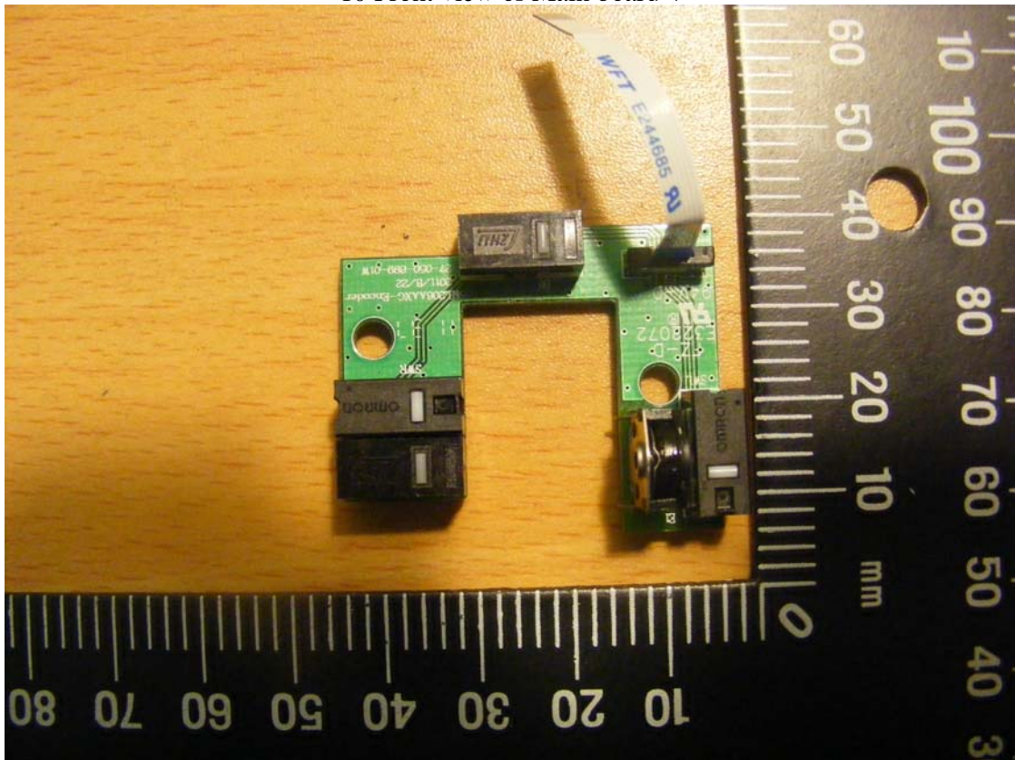
10 Front view of Main board 4
