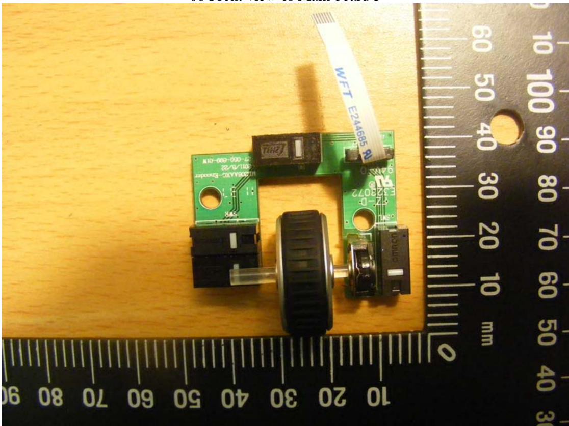
08 Front view of Main board 3
