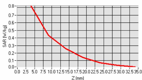
SAR, Z Axis Scan (X = -17, Y = 5)
