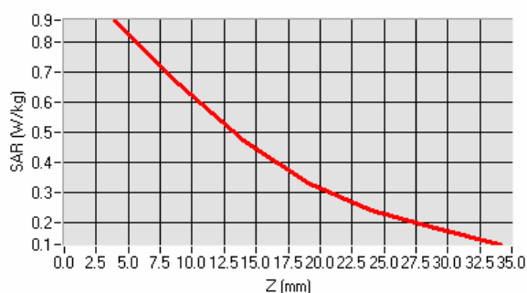
SAR, Z Axis Scan (X = -15, Y = -6)
