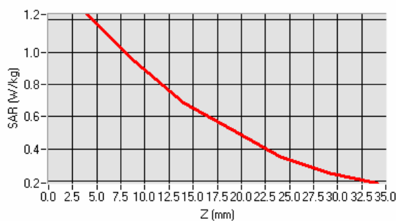
SAR, Z Axis Scan (X = -23, Y = -8)
