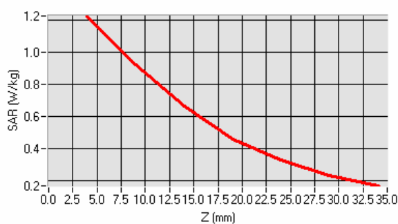
SAR, Z Axis Scan (X = -20, Y = -9)
