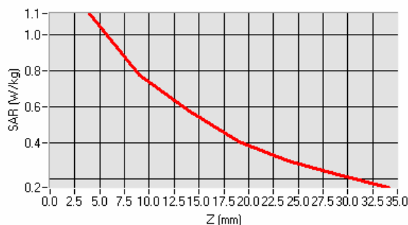
SAR, Z Axis Scan (X = -21, Y = -7)
