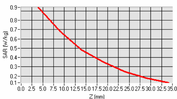
SAR, Z Axis Scan (X = -16, Y = -3)
