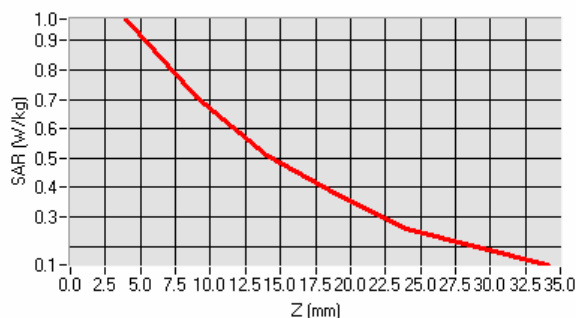
SAR, Z Axis Scan (X = -15, Y = -5)
