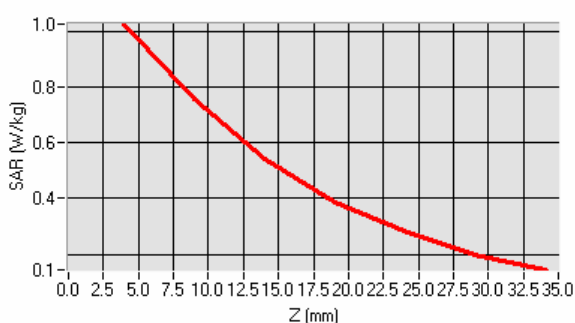
SAR, Z Axis Scan (X = -14, Y = -5)
