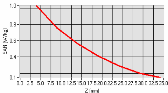
SAR, Z Axis Scan (X = -17, Y = -6)
