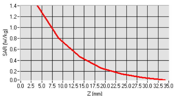
SAR, Z Axis Scan (X = -22, Y = 0)
