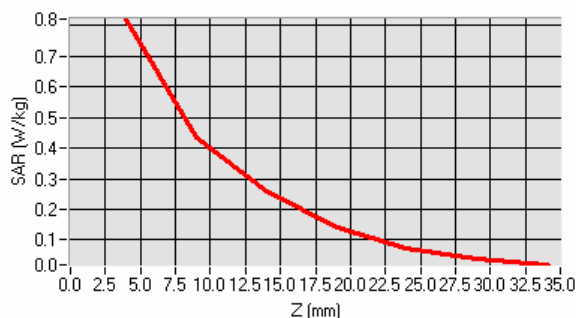
SAR, Z Axis Scan (X = -17, Y = 5)
