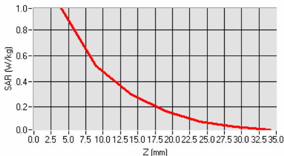
SAR, Z Axis Scan (X = -16, Y = 1)
