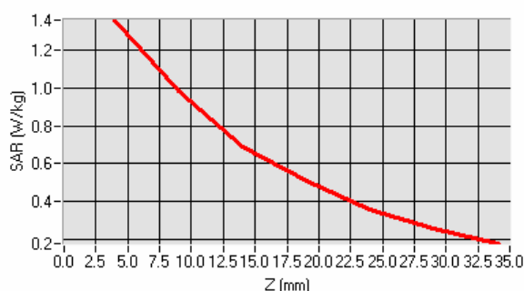
SAR, Z Axis Scan (X = -15, Y = -7)
