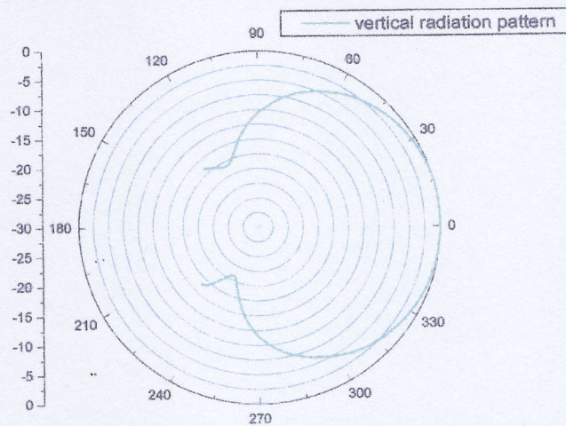
Measured vertical radiation pattern.
