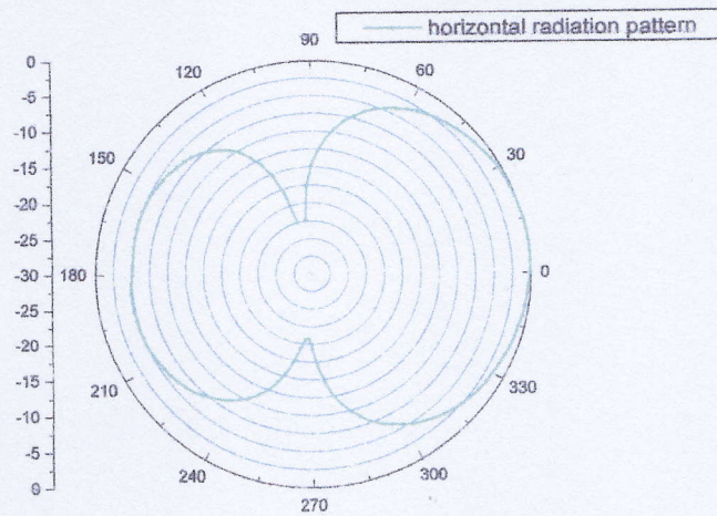
Measured horizontal radiation pattern.
