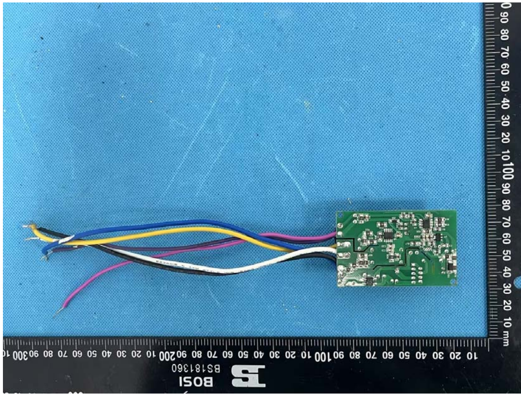
Bluetooth Module, FCC ID: 2ANDL-BT3L
