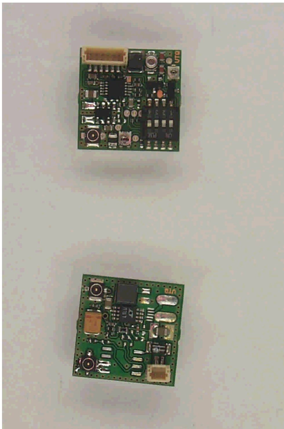
30763TX_PCB2.jpg PCB (transmitter) internal view
