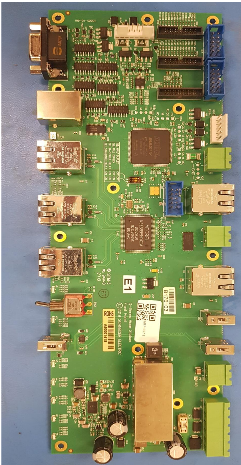
Front Panel PCB Top Layer
