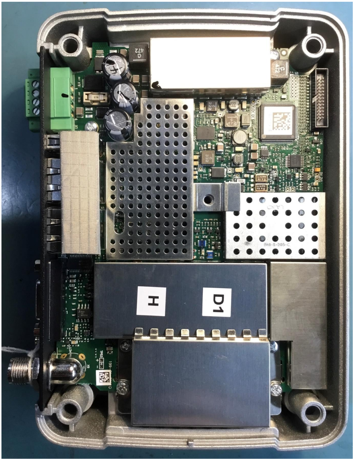
RF Board - Top Shields on
