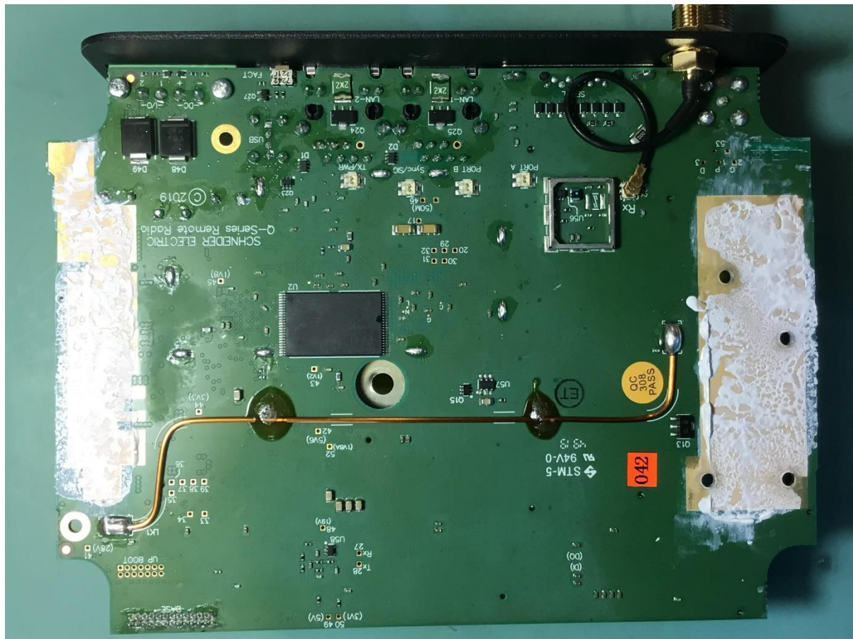
Radio PCB Bottom Layer – Shields off
