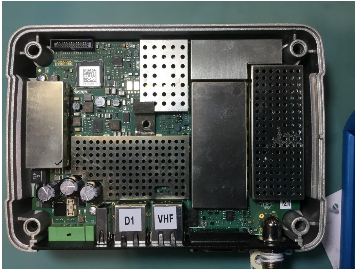
Radio PCB Top Layer (Shields On)
