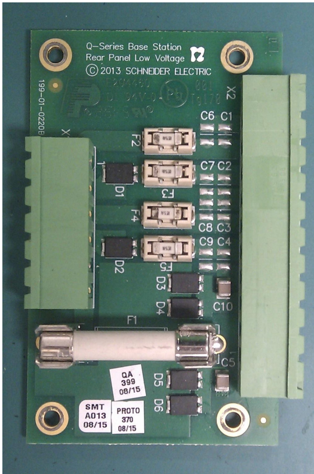
Rear Panel Low Voltage PCB Top Layer
