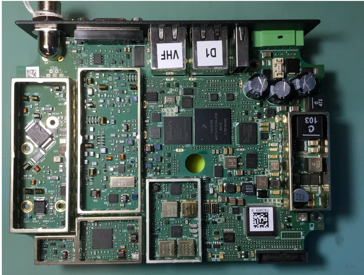
Radio PCB Top Layer (RF Shields Off)
