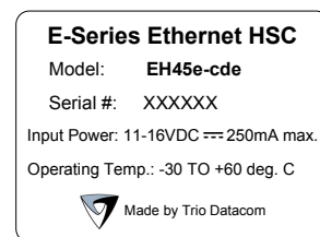
EH45e Ethernet Hot Standby Controller Labels Note the same labels are used for all regions
