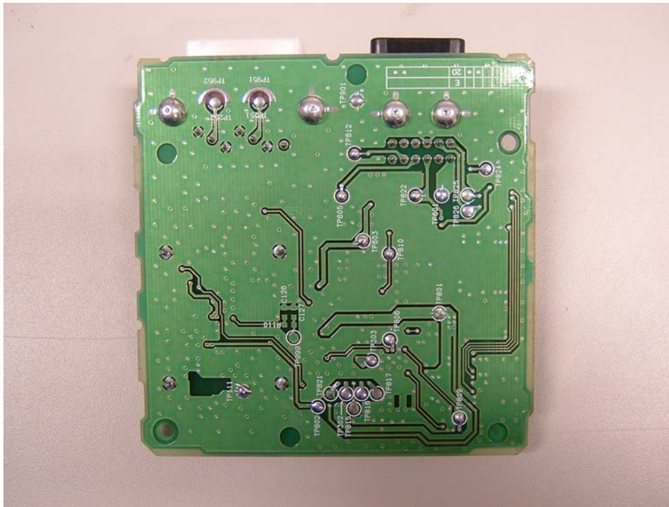
Receiver inside solder side
