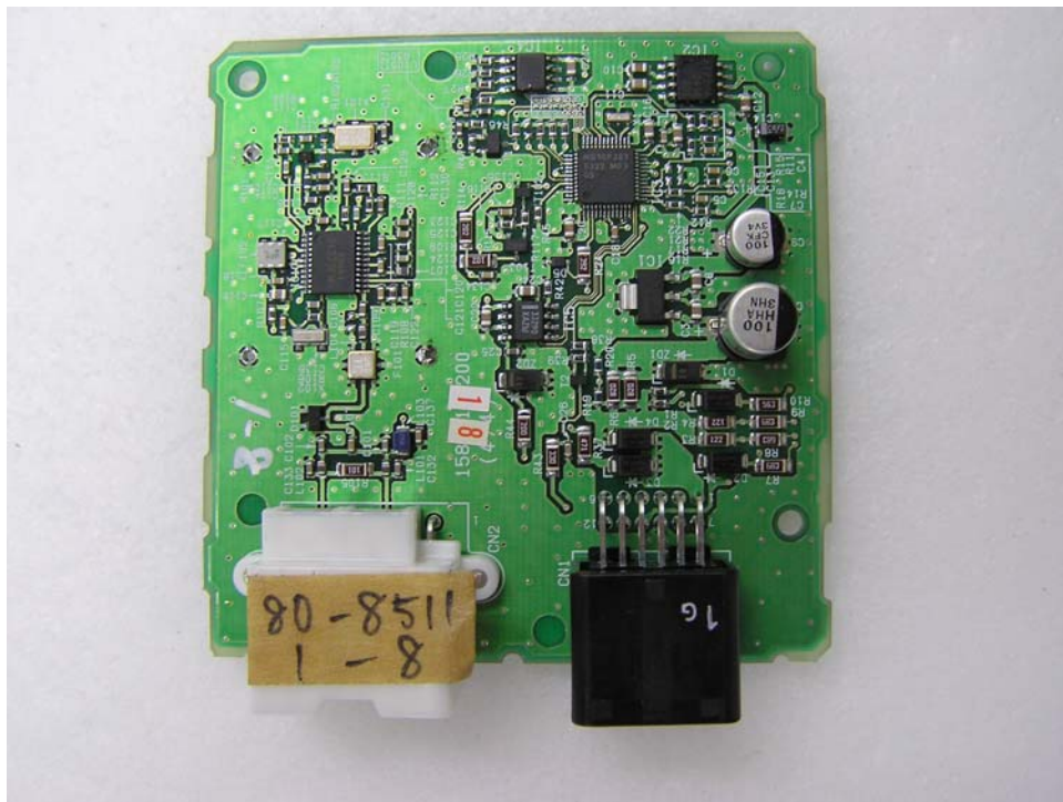
Receiver inside comp side without shield
